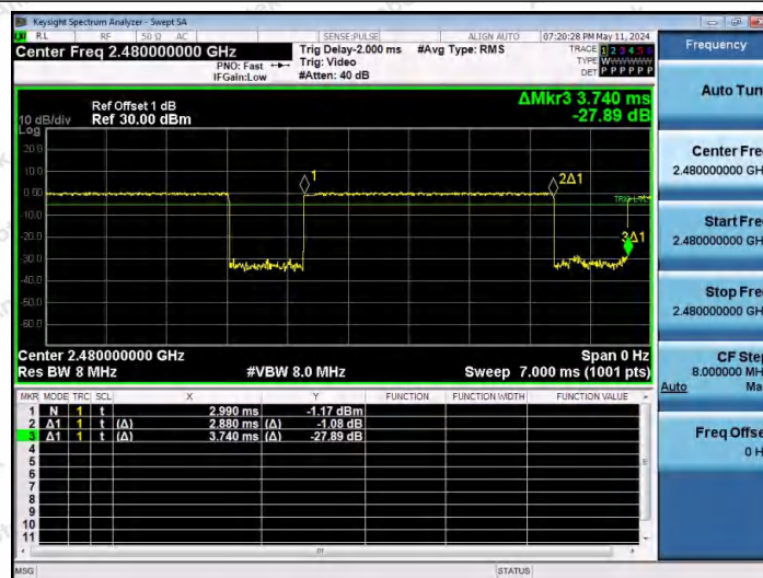
NTNV-3DH5-Ant1-2480
