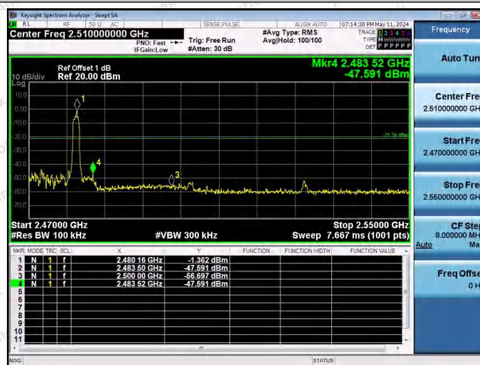
2DH5-Ant1-2480-PASS
