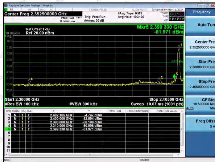
2DH5-Ant1-2402-PASS
