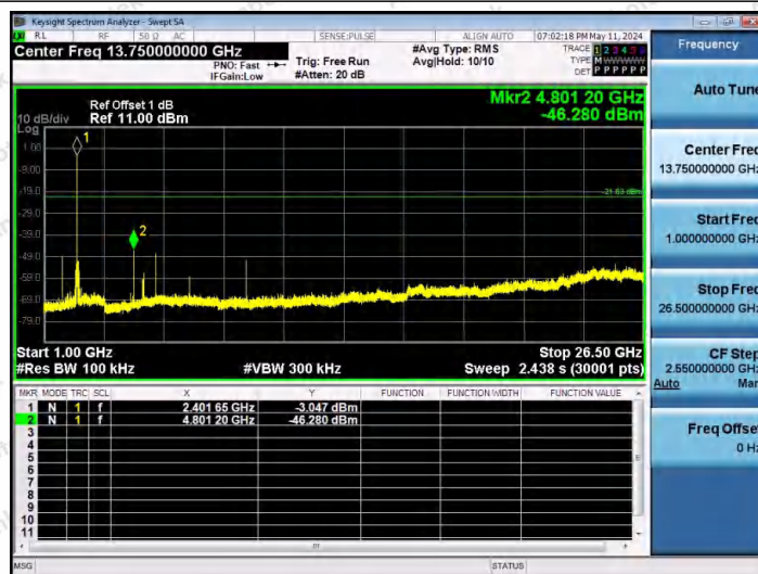
DH5-Ant1-2402-1000~26500-PASS
