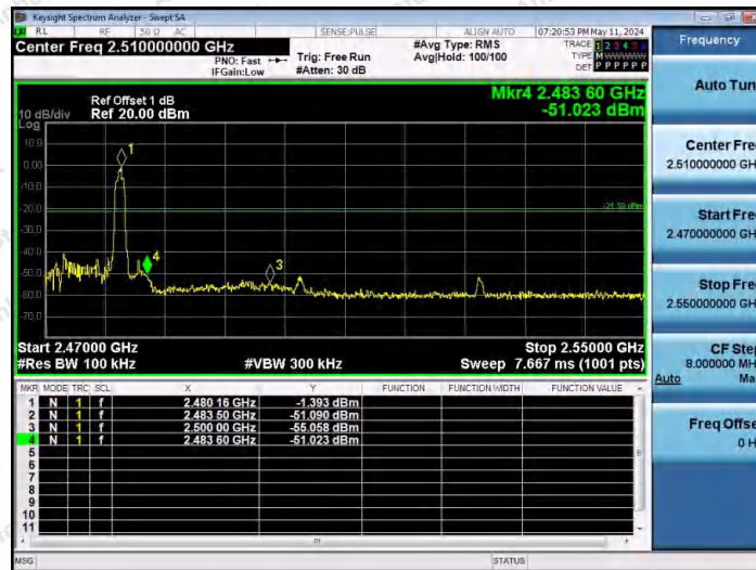
3DH5-Ant1-2480-PASS
