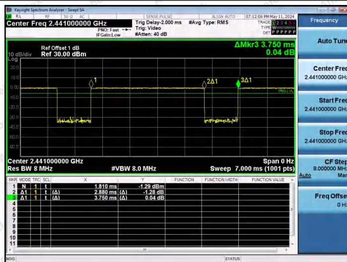
NTVN-2DH5-Ant1-2441
