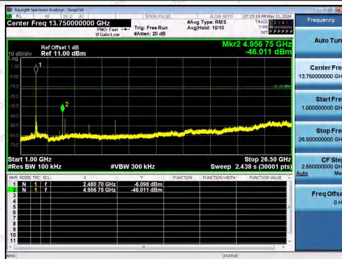
2DH5-Ant1-2480-1000~26500-PASS
