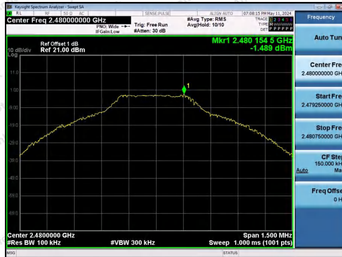
DH5-Ant1-2480-0~Reference-PASS
