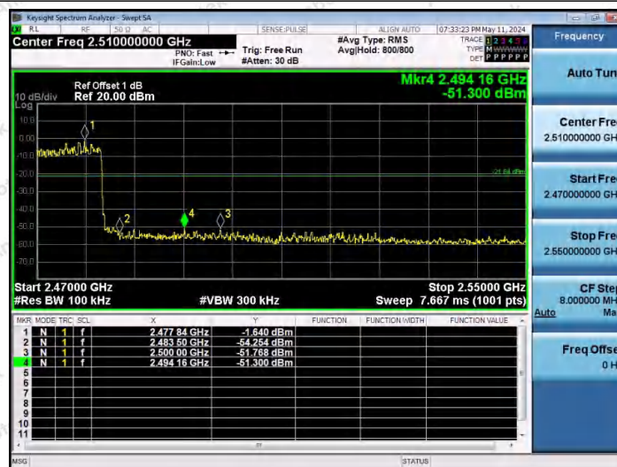
3DH5-Ant1-Hop_2480-PASS
