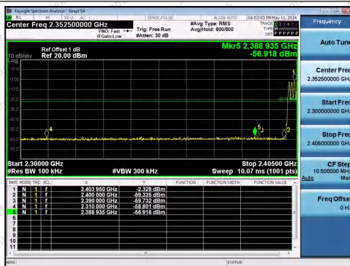
DH5-Ant1-Hop_2402-PASS
