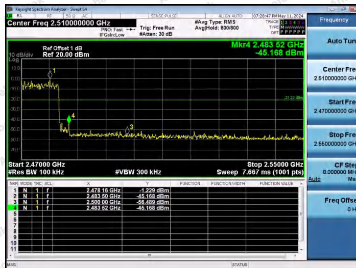
2DH5-Ant1-Hop_2480-PASS
