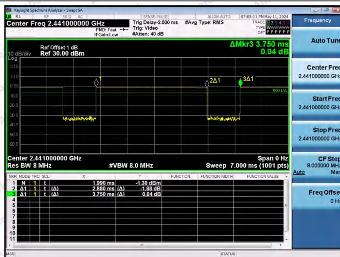
NTNV-DH5-Ant1-2441
