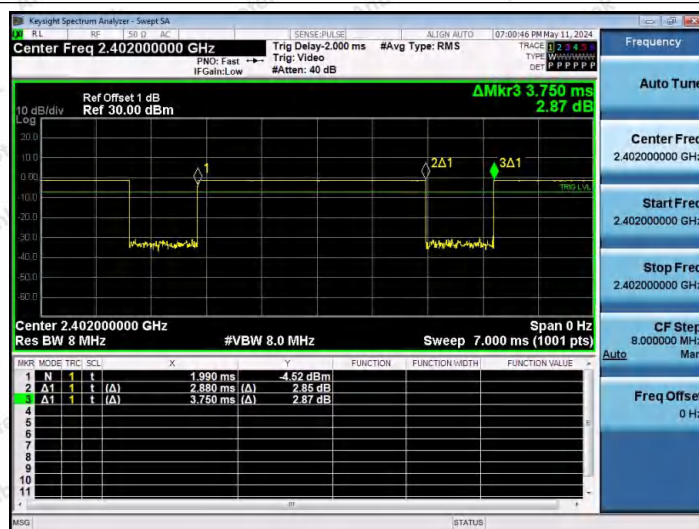
NTNV-DH5-Ant1-2402
