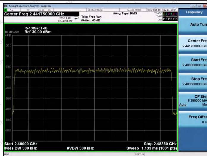
3DH5-Ant1-Hop-PASS
