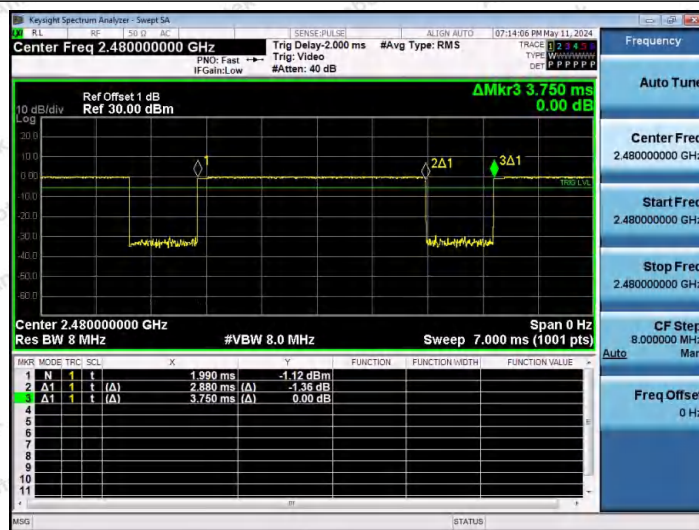
NTVN-2DH5-Ant1-2480
