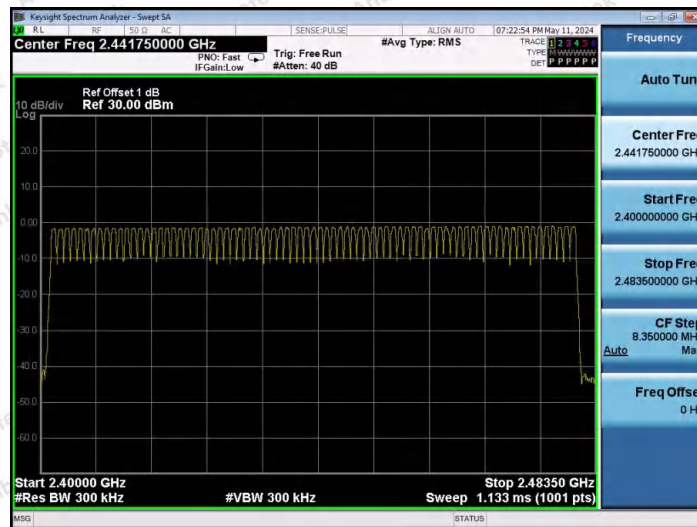
DH5-Ant1-Hop-PASS
