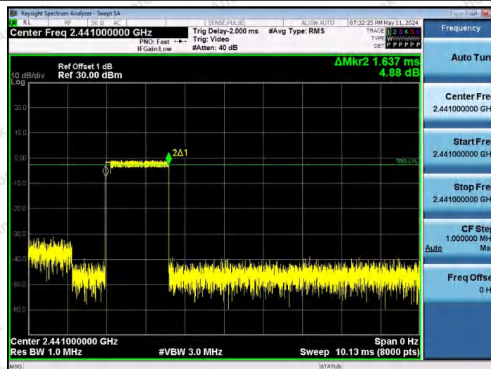
2DH3-Ant1-Hop-PASS
