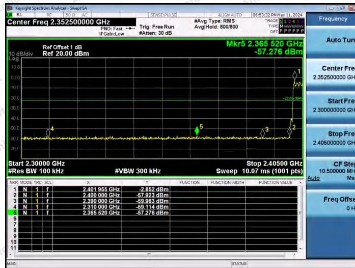
2DH5-Ant1-Hop_2402-PASS
