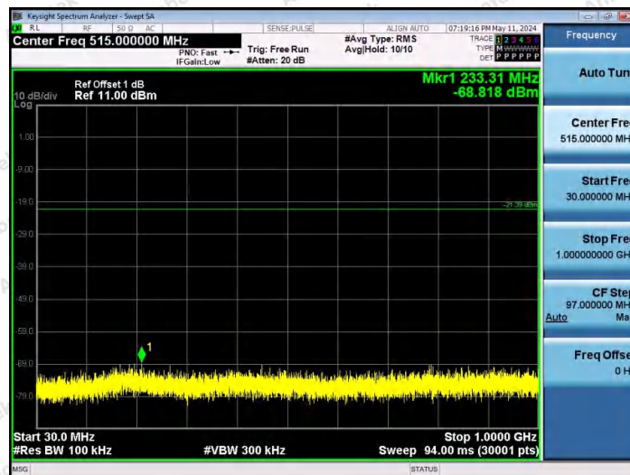
3DH5-Ant1-2441-30~1000-PASS
