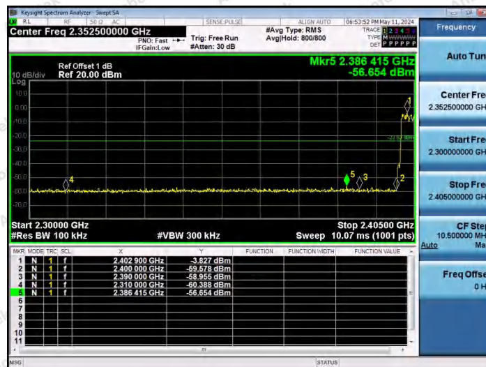
3DH5-Ant1-Hop_2402-PASS
