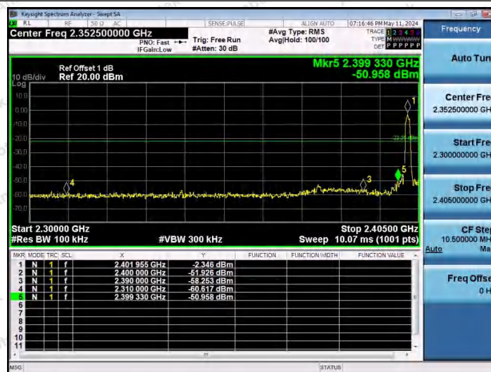
3DH5-Ant1-2402-PASS
