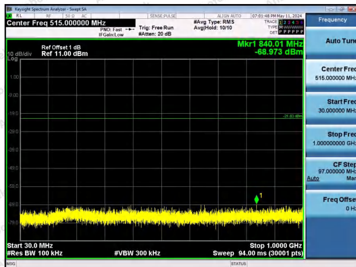
DH5-Ant1-2402-30~1000-PASS
