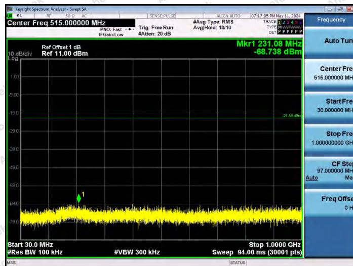
3DH5-Ant1-2402-30~1000-PASS
