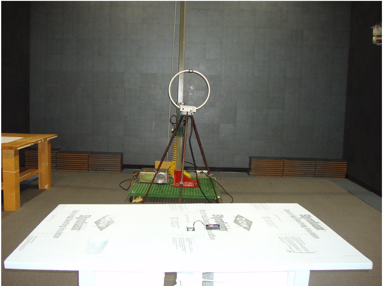
Photo 4 – Rear View of the Radiated Emissions Test Set-up below 30 MHz
