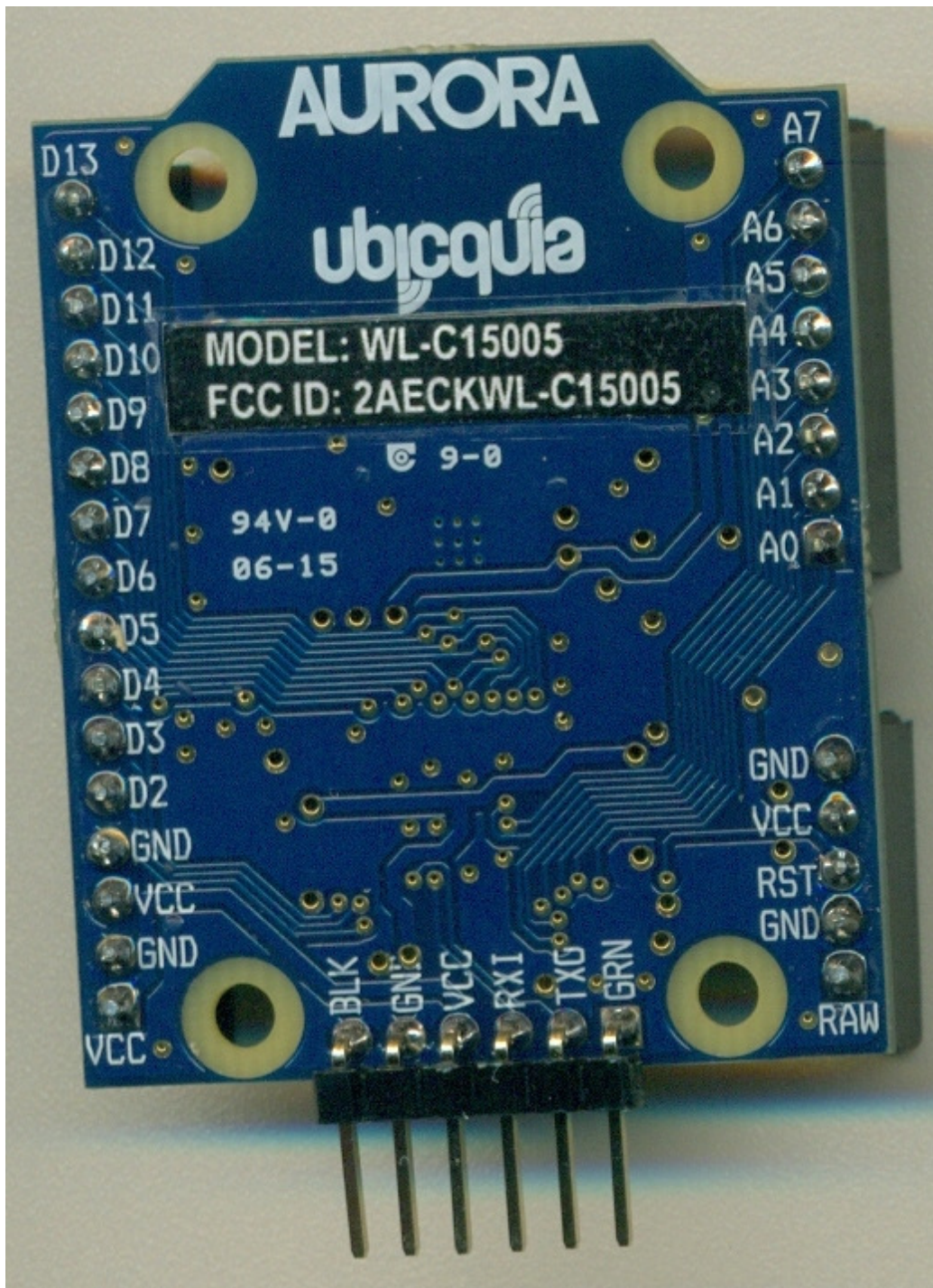
Photo 3 – Bottom View
