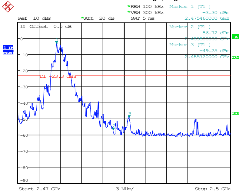
GFSK: Band Edge, Right Side
