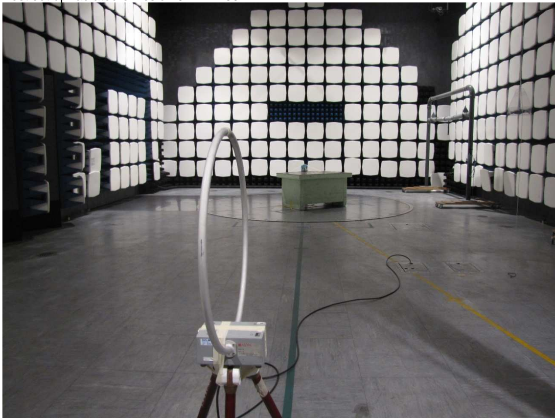
Test set up radiated emission 9 kHz – 30 MHz
