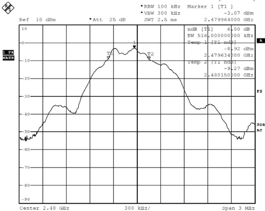
6dB Bandwidth of Fundamental Emission on GFSK (2480MHz)
