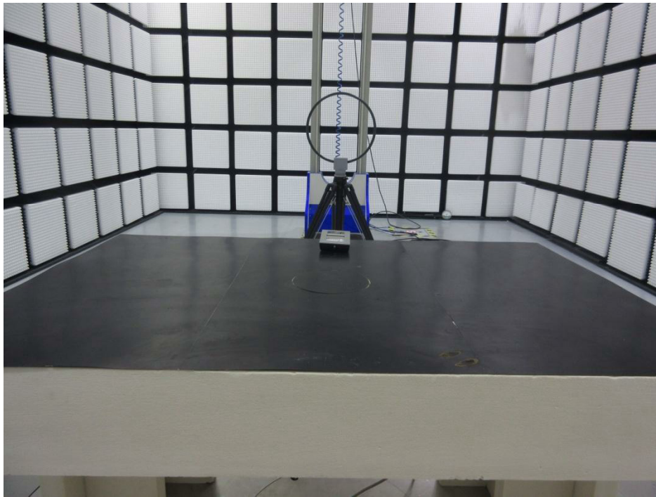
Setup photo of radiated emission (9KHz-30MHz)
