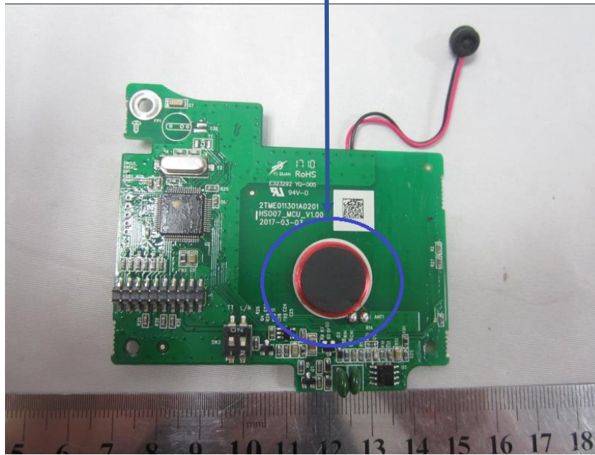
Coil Antenna
