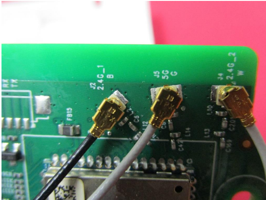
WIFI antenna
