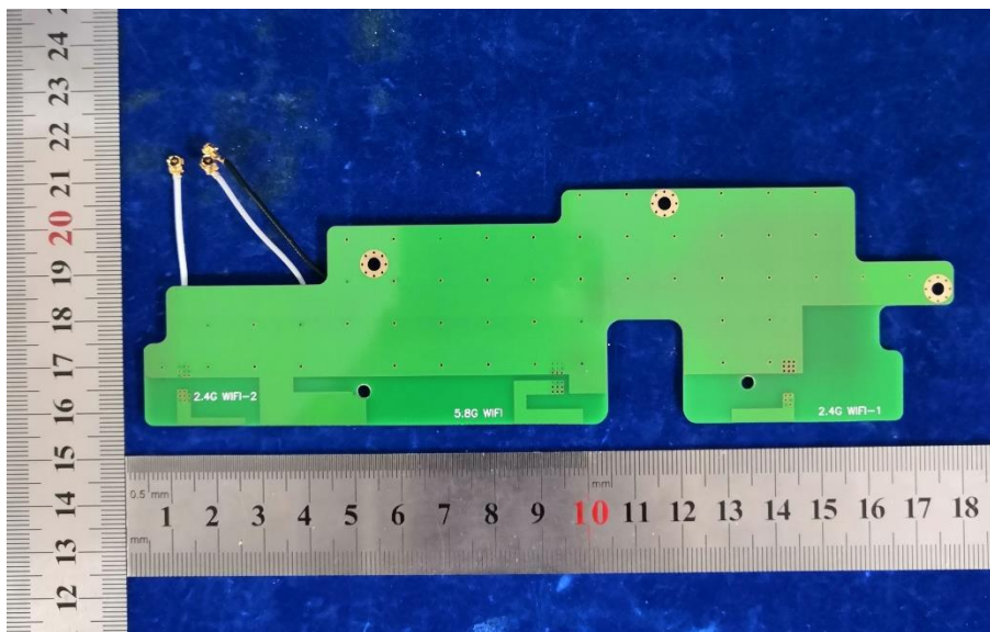
WIFI antenna
