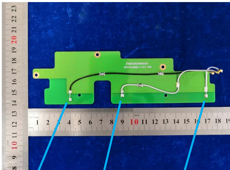
Antenna 2.4G-1
