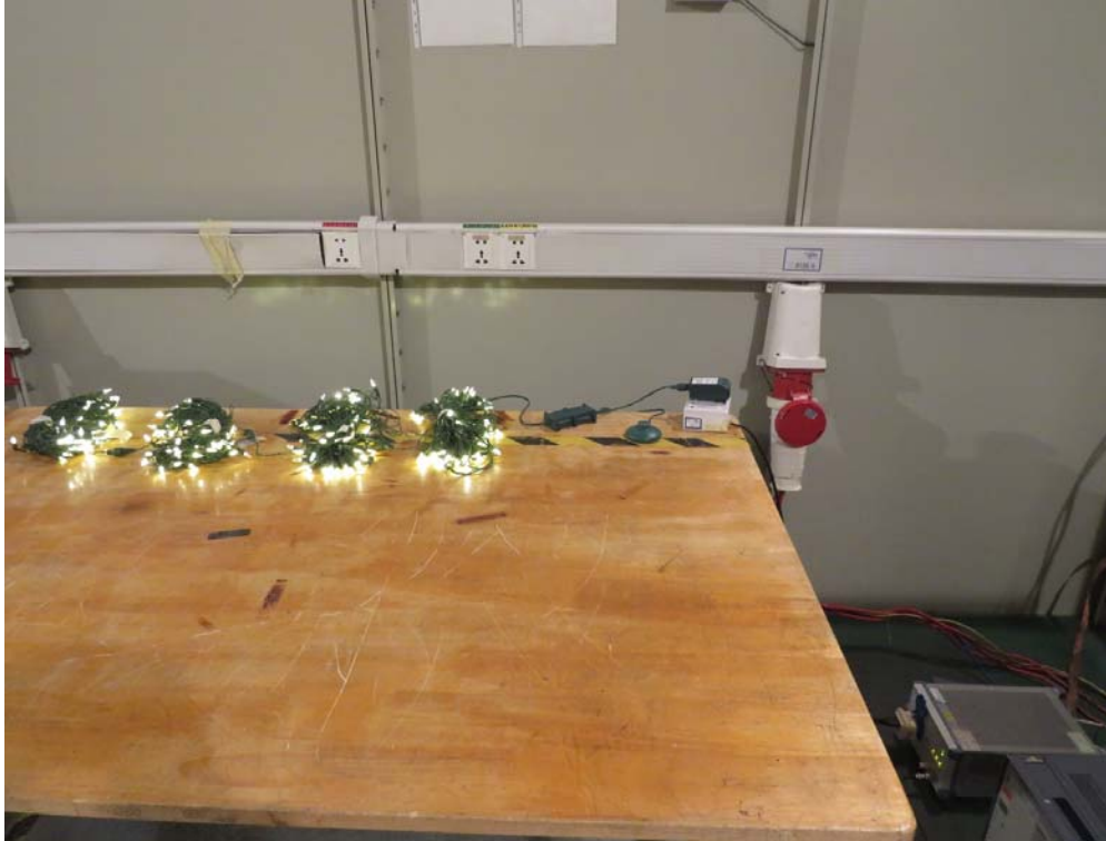
Conducted Emission
