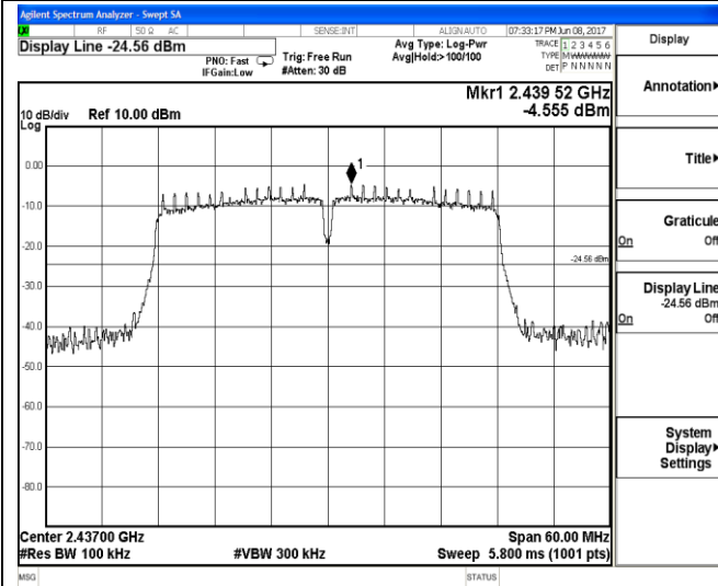
2407 MHz – 2467 MHz
