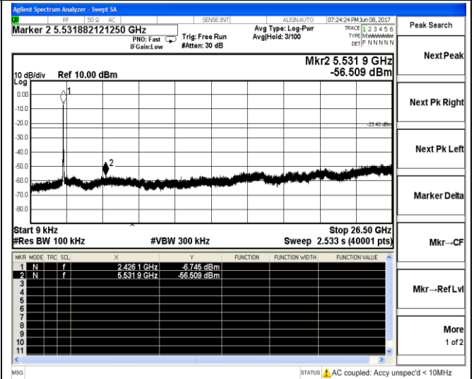
9 KHz – 26.5 GHz
