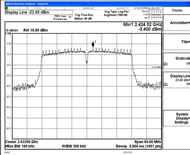
2392 MHz – 2452 MHz
