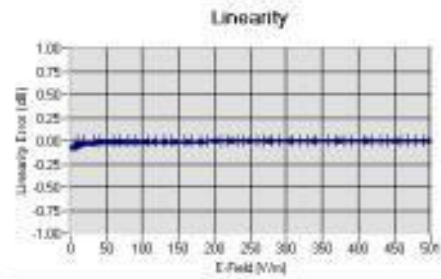
Linearity: \pm 1.09\% ( \pm 0.07\text{dB} )
