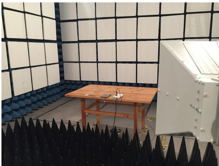
Radiated Test 8
