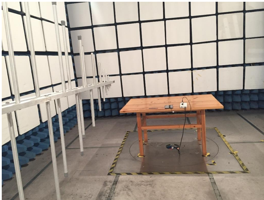
Radiated Test 7
