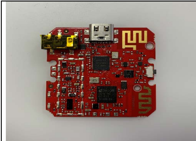
Tx-Top View
