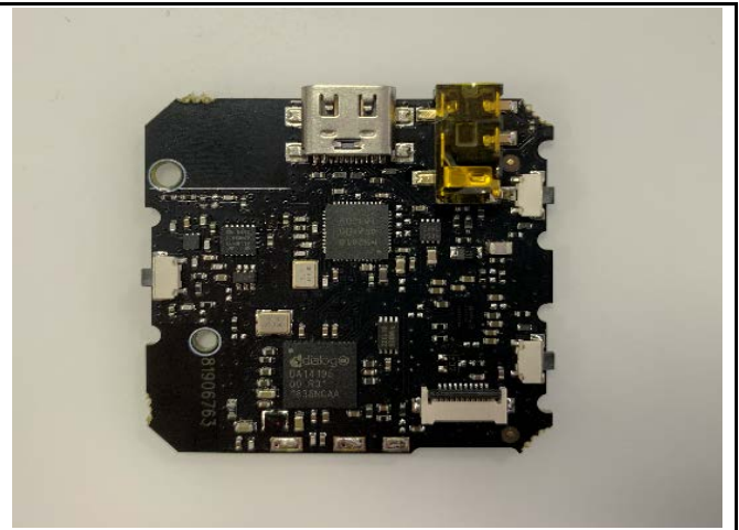
Rx-Top View
