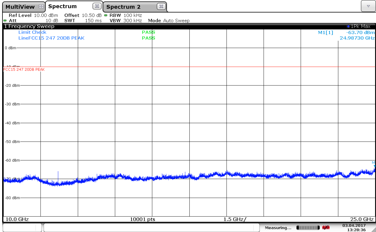
Conducted Emissions, 10000 – 25000 MHz, 2441MHz
