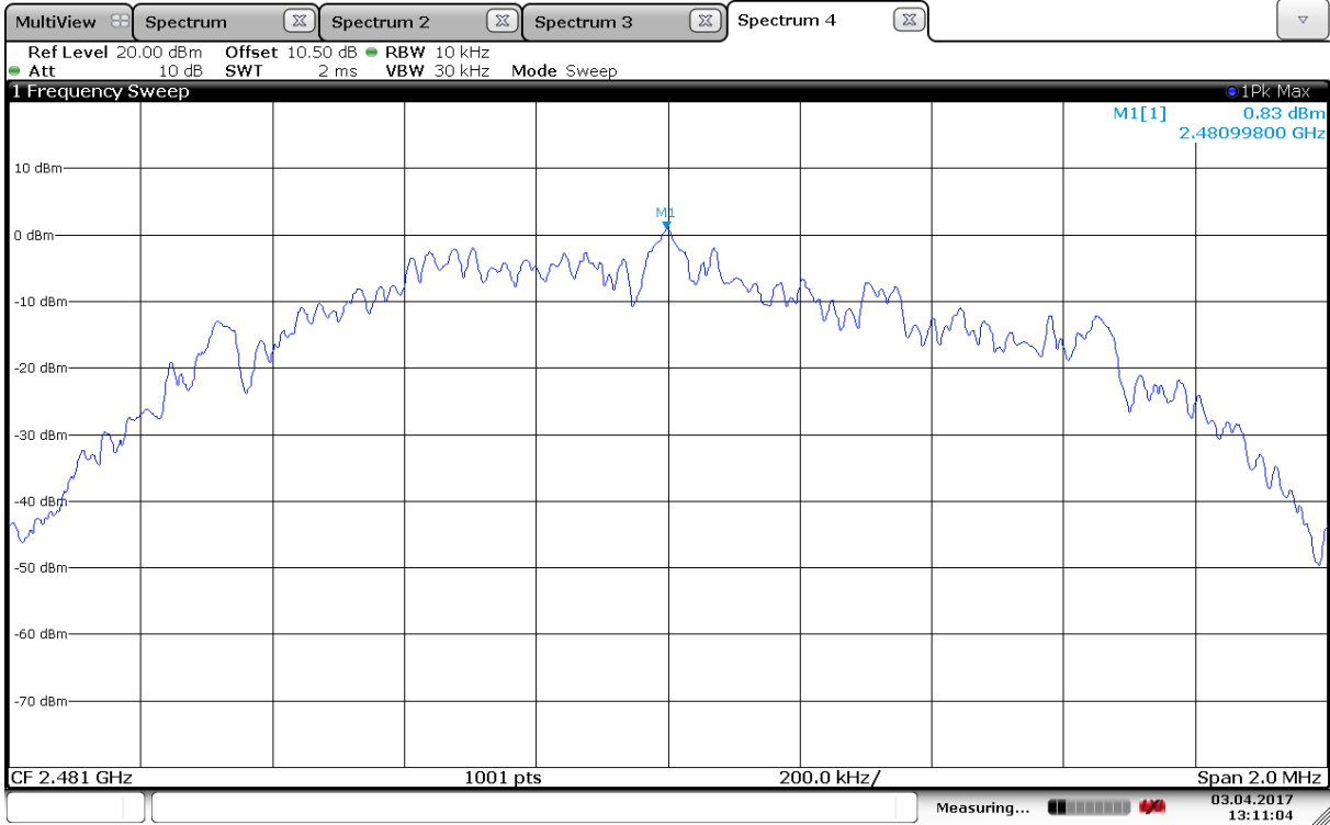
PSD, 2481MHz
