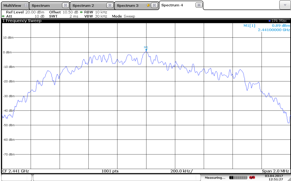
PSD, 2441MHz
