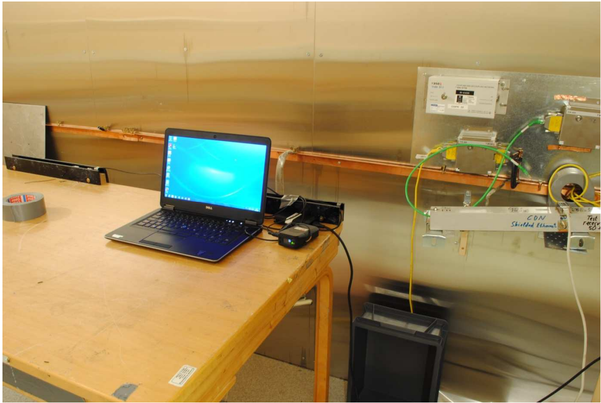
Conducted Emissions
