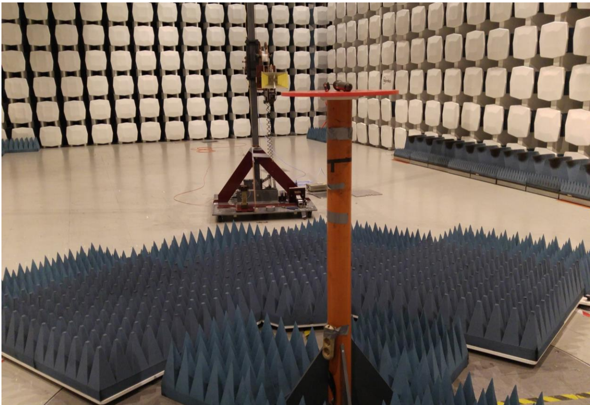
Radiated emissions, 1 – 8.5 GHz
