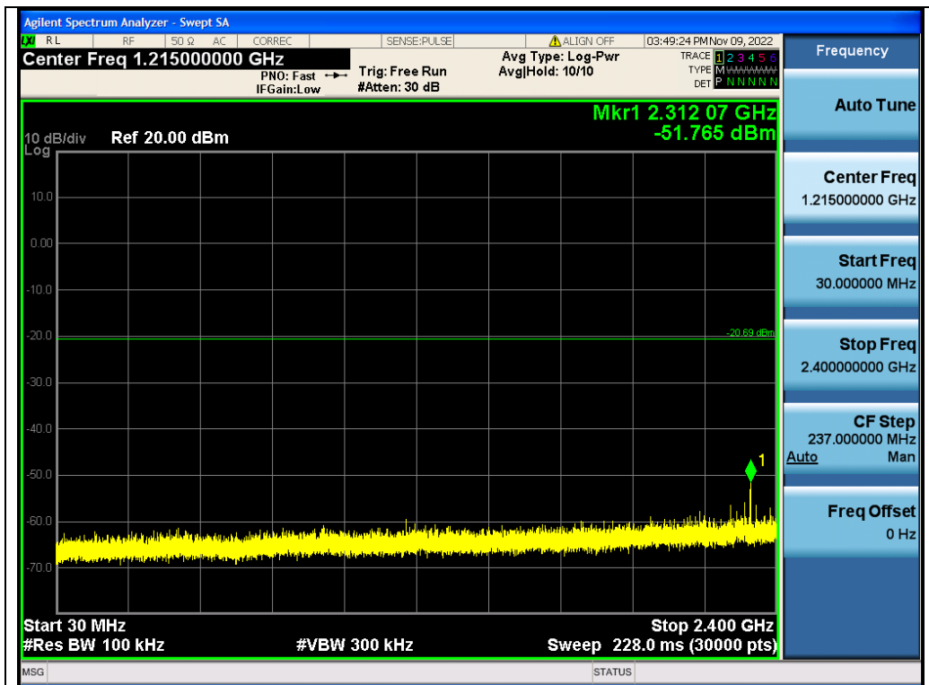
Test_Graph_2.4G_ANT1_2440_1Mbps_Lower Band Emissions
