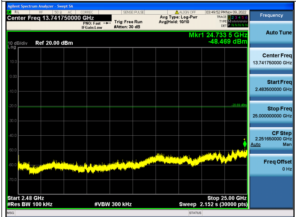
Test_Graph_2.4G_ANT1_2440_1Mbps_Higher Band Emissions
