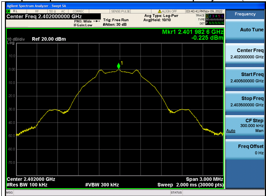
Test_Graph_2.4G_ANT1_2402_1Mbps_Reference Level
