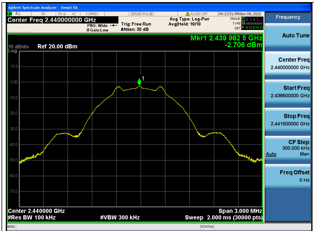
Test_Graph_2.4G_ANT2_2440_1Mbps_Reference Level
