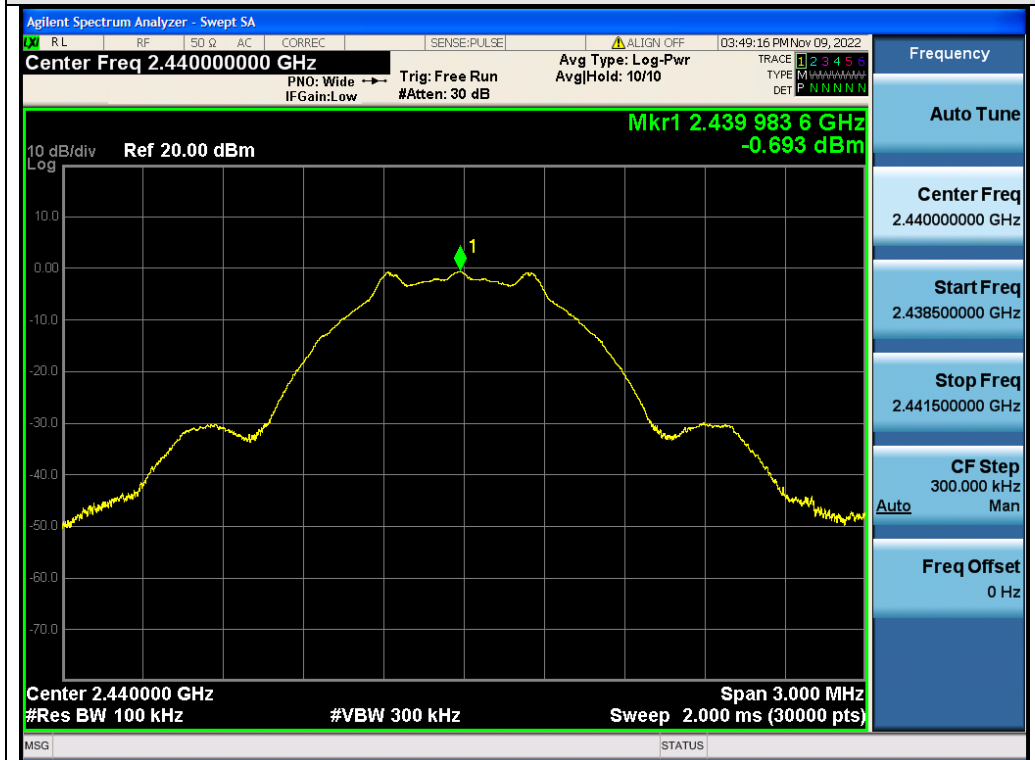
Test_Graph_2.4G_ANT1_2440_1Mbps_Reference Level
