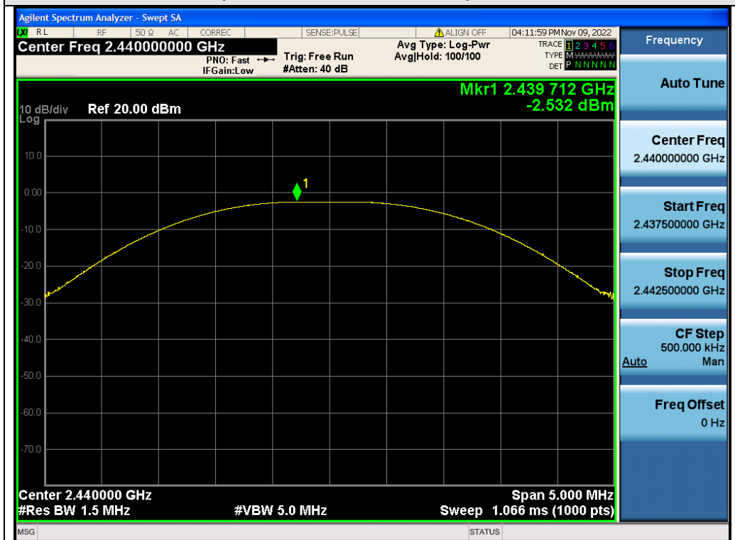
Test_Graph_2.4G_ANT2_2440_1Mbps_Peak Power
