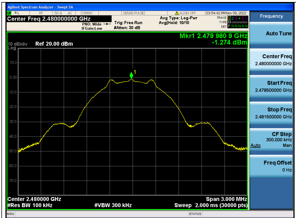
Test_Graph_2.4G_ANT1_2480_1Mbps_Reference Level
