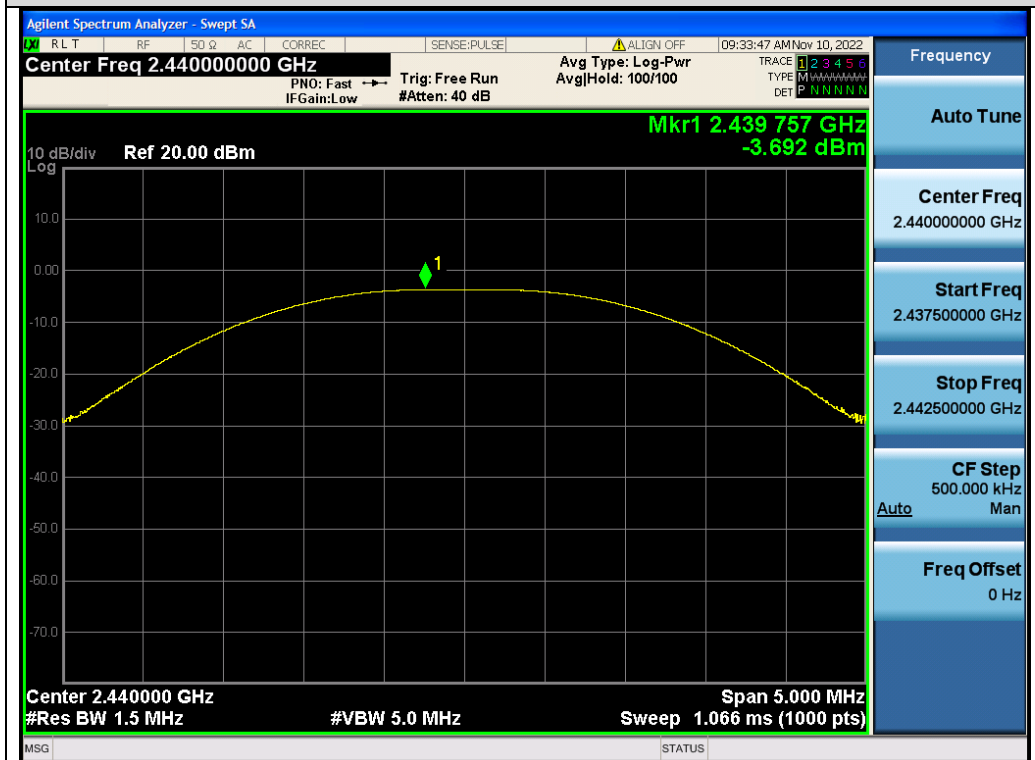
Test_Graph_GFSK_ANT2_2440_Peak Power
