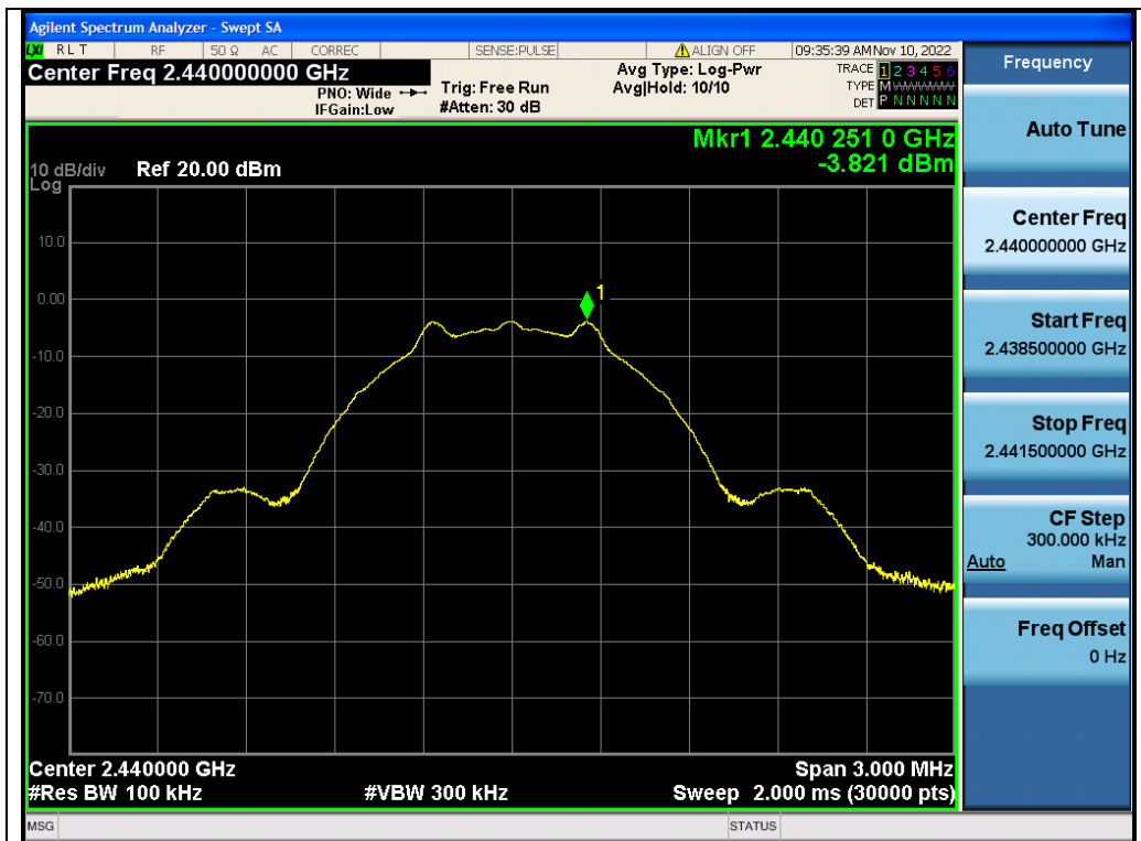
Test_Graph_GFSK_ANT2_2440_Reference Level
