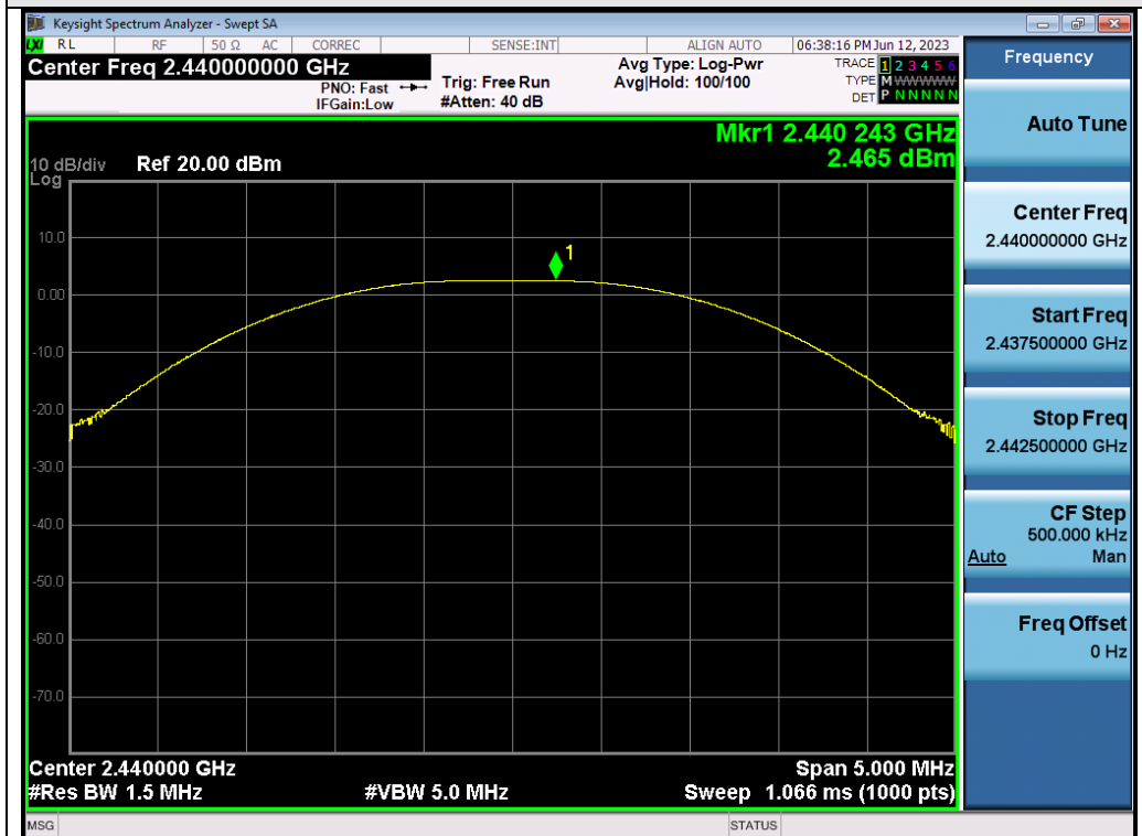
Test_Graph_ANT2_2440_Peak Power
