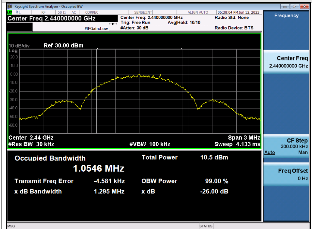
Test_Graph_ANT2_2440_OBW
