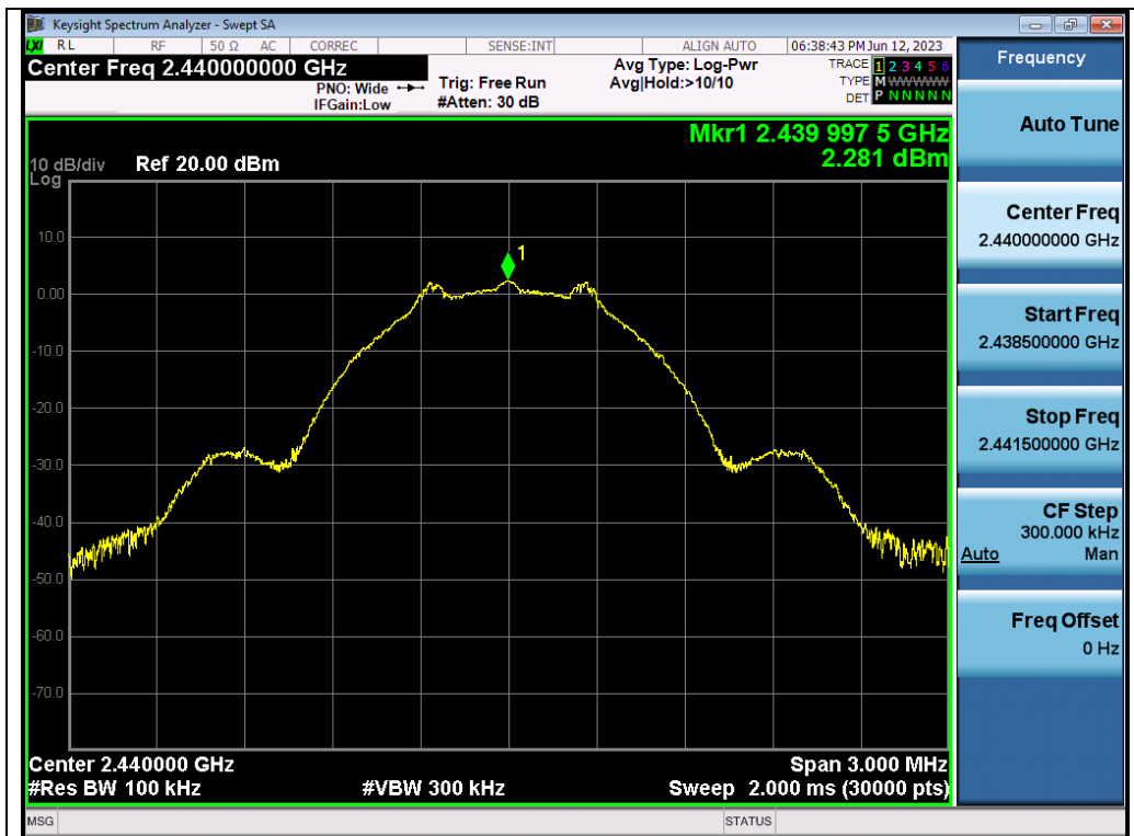
Test_Graph_ANT2_2440_Reference Level
