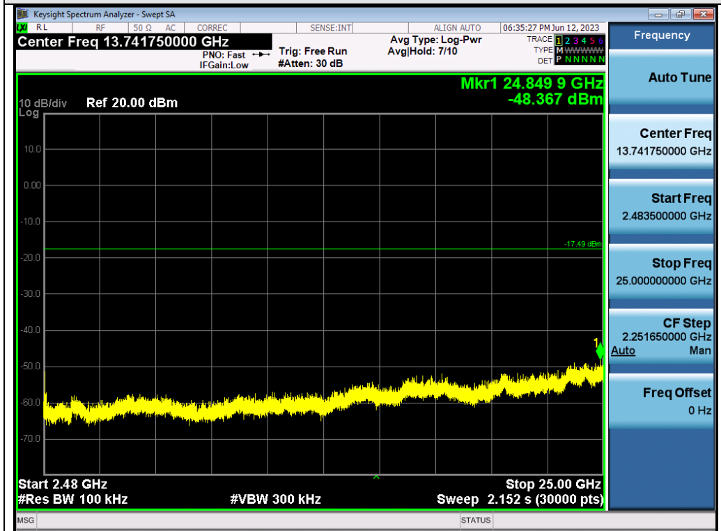
Test_Graph_ANT2_2402_Higher Band Emissions
