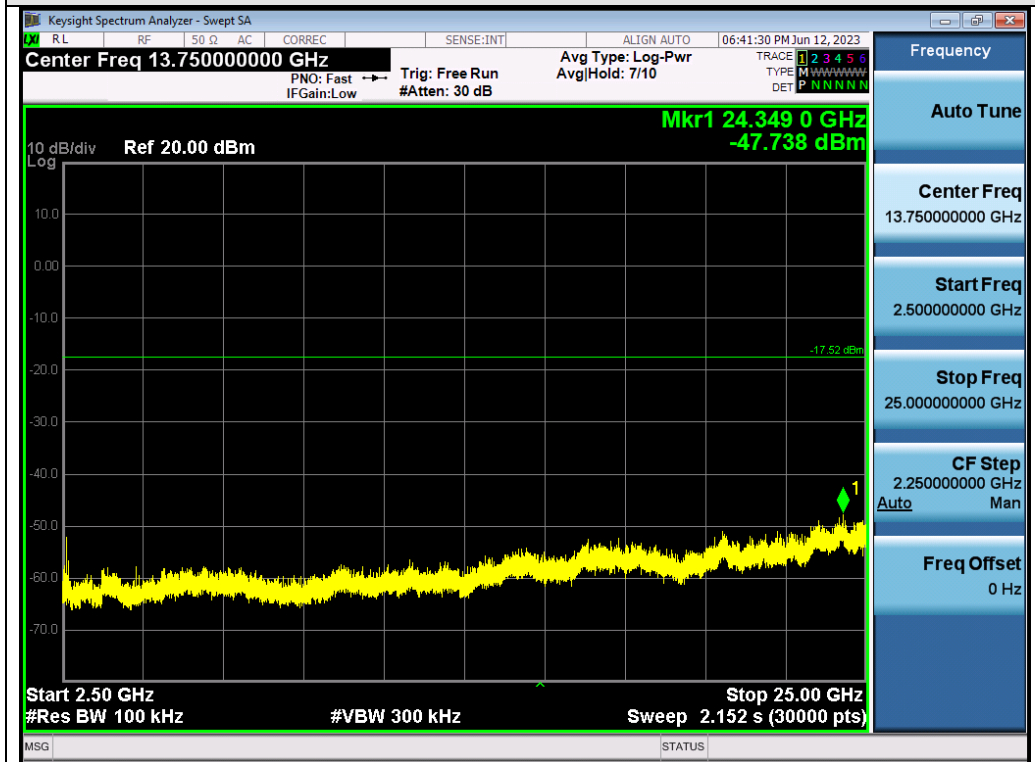
Test_Graph_ANT2_2480_Higher Band Emissions
