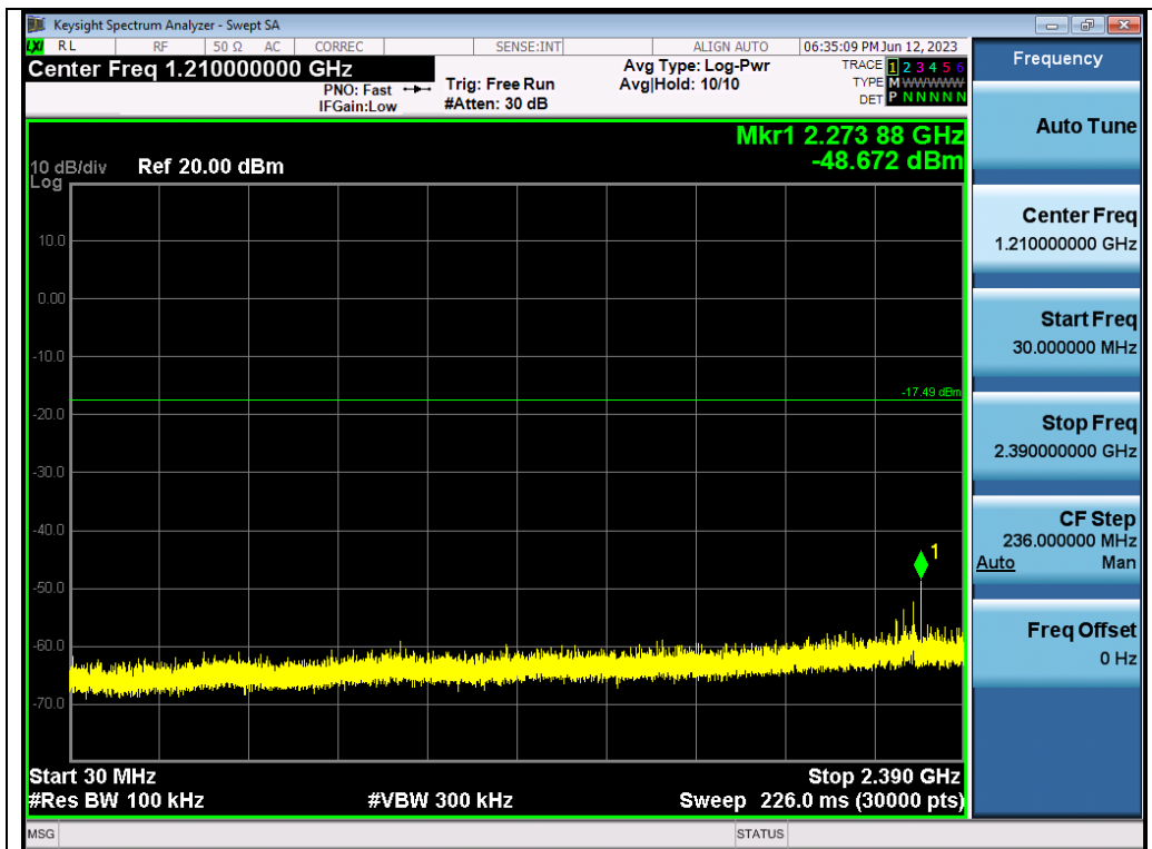
Test_Graph_ANT2_2402_Lower Band Emissions
