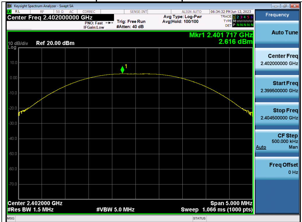
Test_Graph_ANT2_2402_Peak Power
