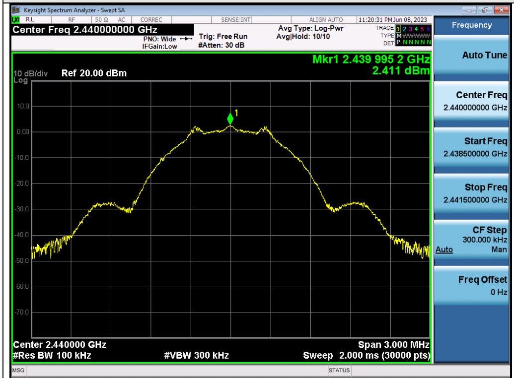
Test_Graph_ANT1_2440_Reference Level
