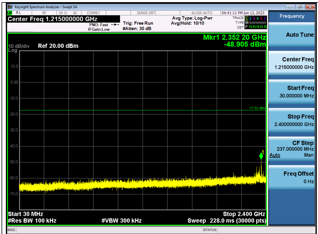
Test_Graph_ANT2_2480_Lower Band Emissions
