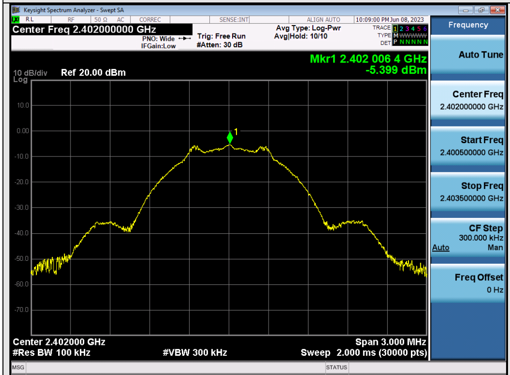
Test_Graph_ANT2_2402_Reference Level
