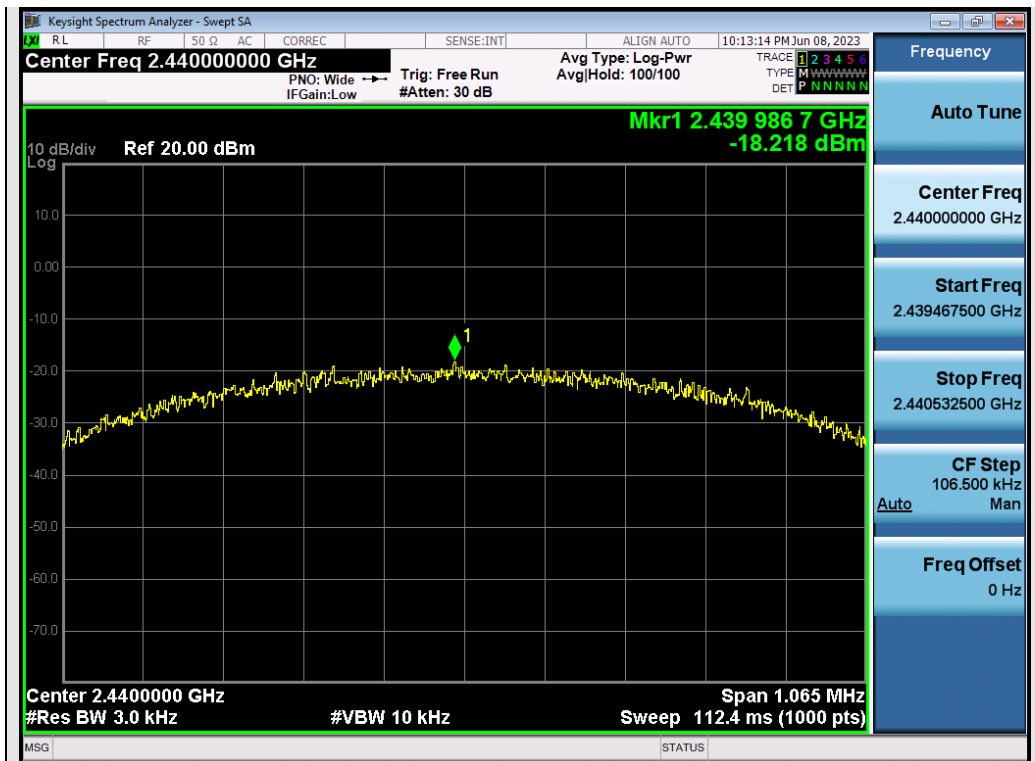
Test_Graph_ANT2_2440_PSD
