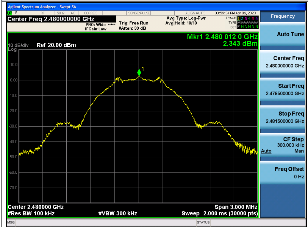
Test_Graph_LE1M_ANT2_2480_1Mbps_Reference Level
