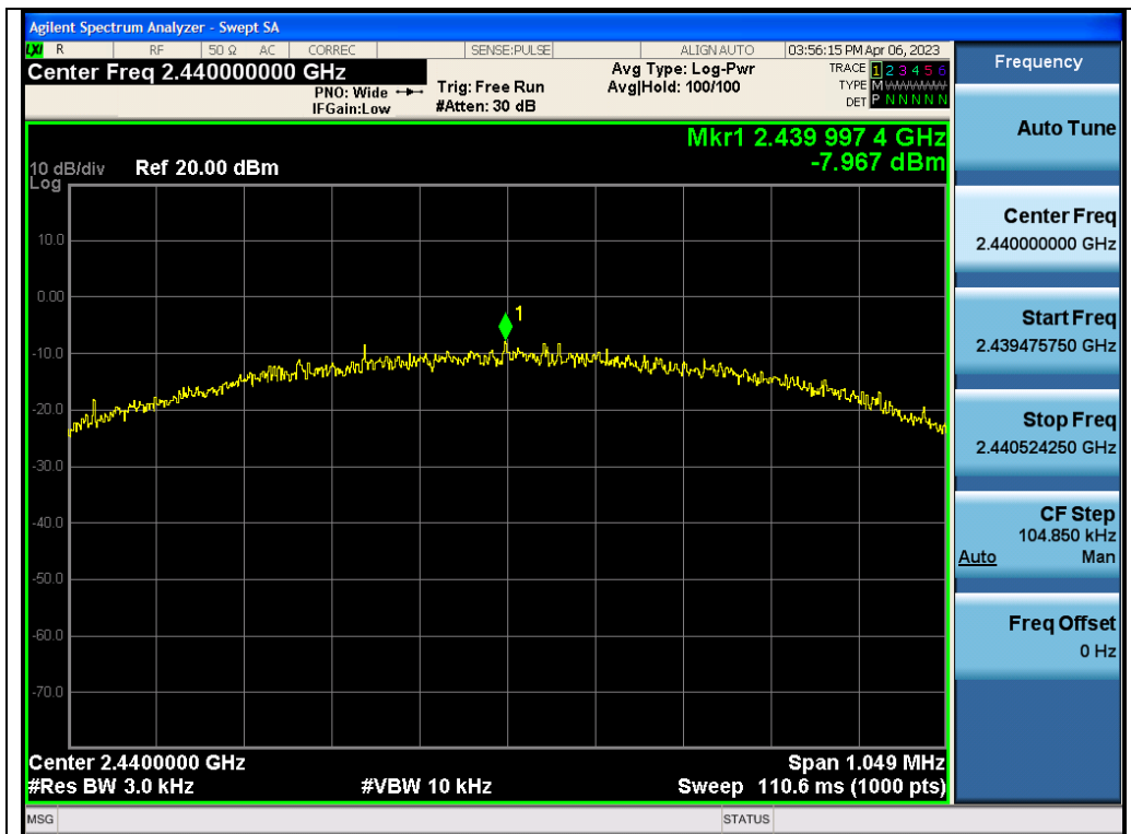
Test_Graph_LE1M_ANT2_2440_1Mbps_PSD
