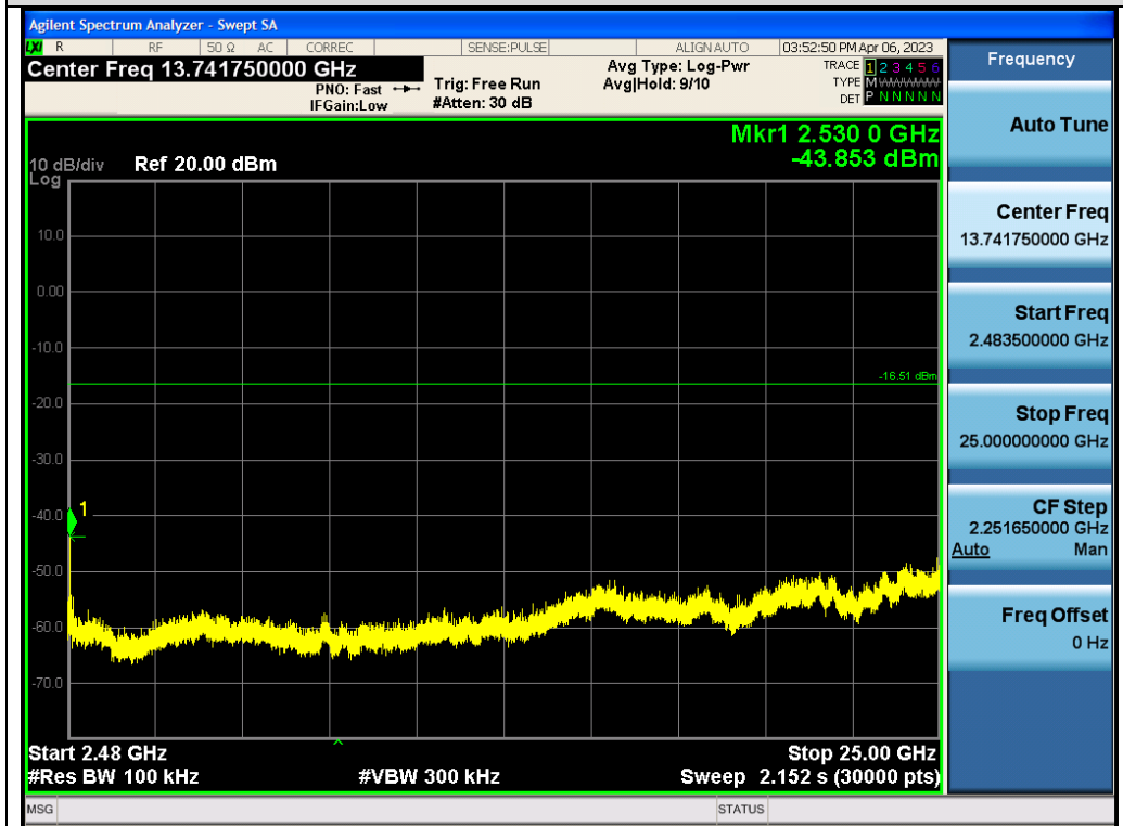
Test_Graph_LE1M_ANT2_2402_1Mbps_Higher Band Emissions
