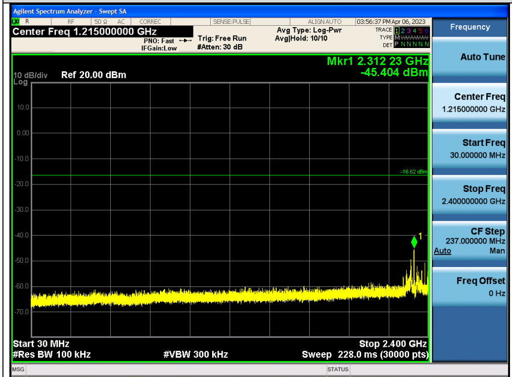
Test_Graph_LE1M_ANT2_2440_1Mbps_Lower Band Emissions
