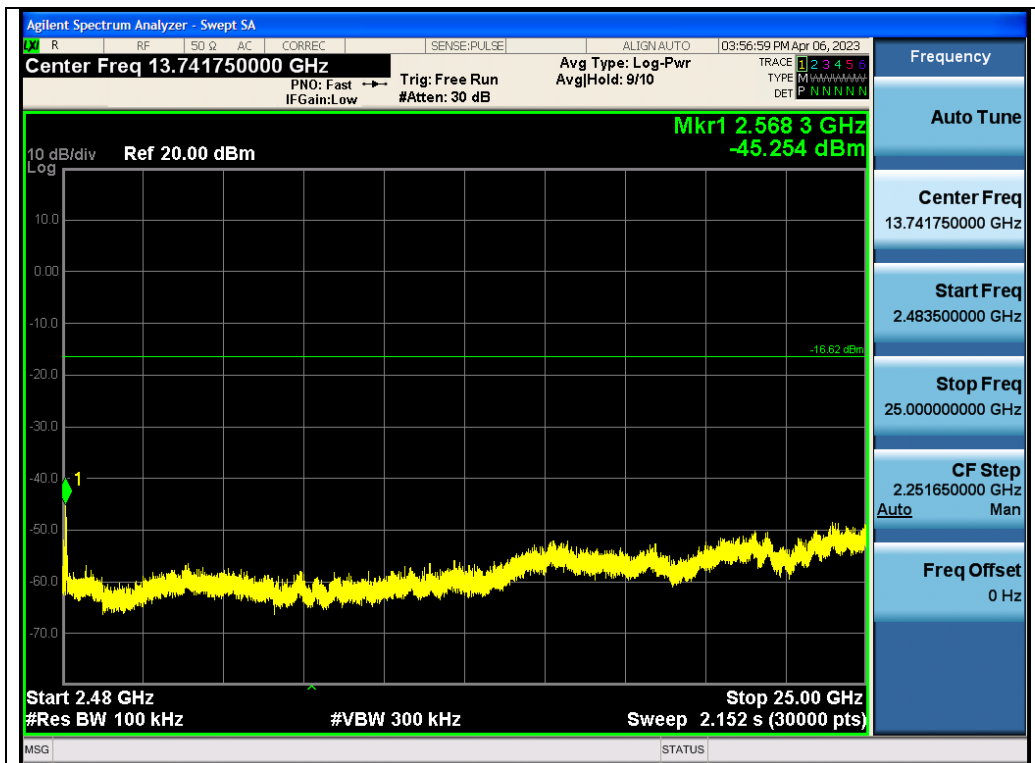
Test_Graph_LE1M_ANT2_2440_1Mbps_Higher Band Emissions
