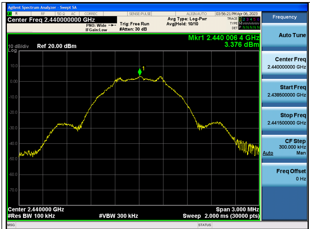
Test_Graph_LE1M_ANT2_2440_1Mbps_Reference Level
