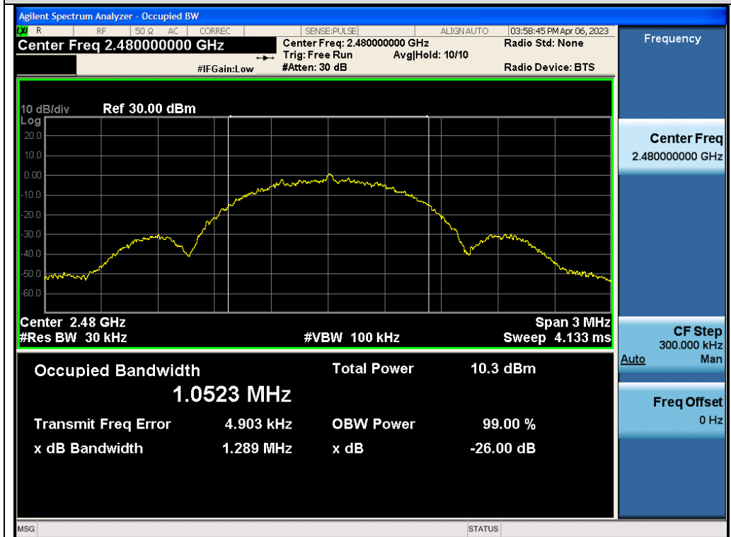
Test_Graph_LE1M_ANT2_2480_1Mbps_OBW
