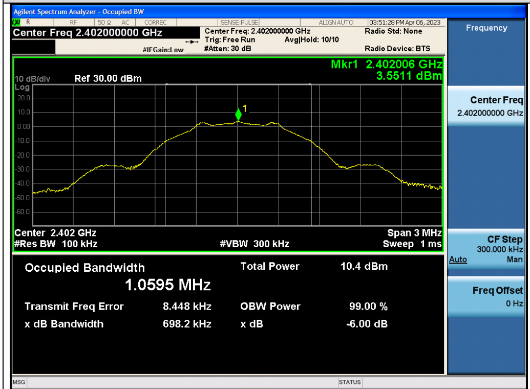
Test_Graph_LE1M_ANT2_2402_1Mbps_DTSBW
