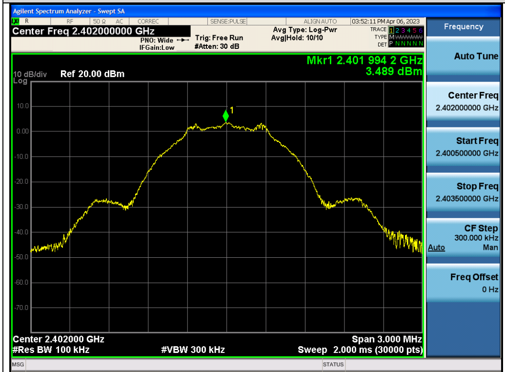
Test_Graph_LE1M_ANT2_2402_1Mbps_Reference Level
