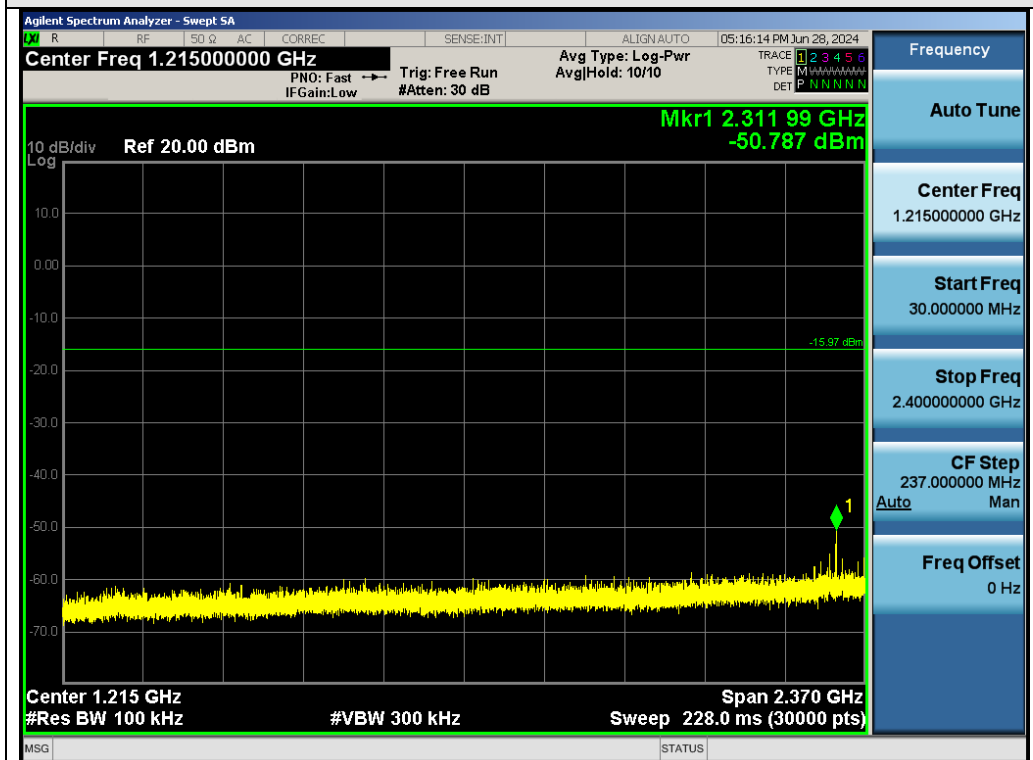
Test_Graph_GFSK_ANT2_2440_Lower Band Emissions
