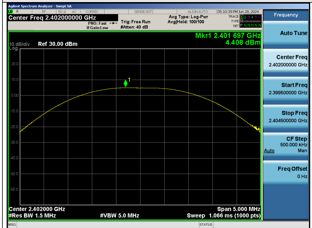
Test_Graph_GFSK_ANT2_2402_Peak Power
