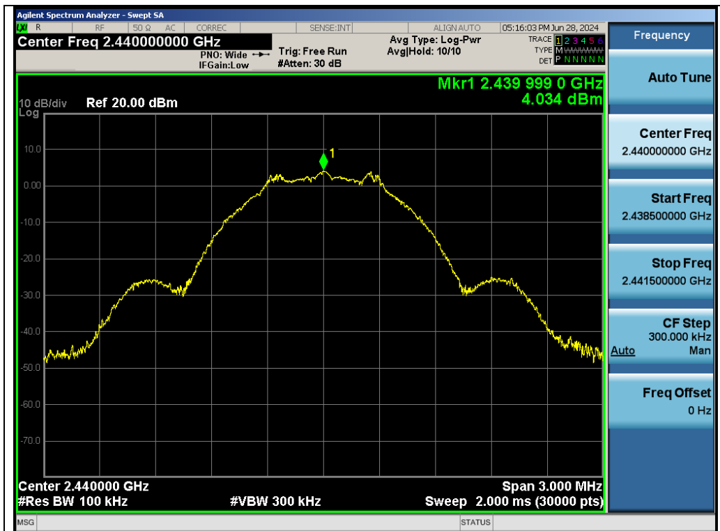
Test_Graph_GFSK_ANT2_2440_Reference Level
