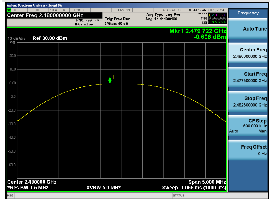
Test_Graph_GFSK_ANT2_2480_Peak Power
