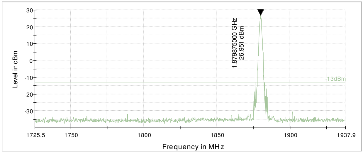
PK+_CLRWR@1GHz-3GHz_LTE B2 MID CH -13dBm
