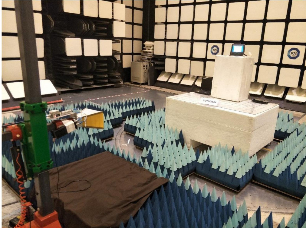
Receiver Spurious Emissions Test Setup (Front View)
