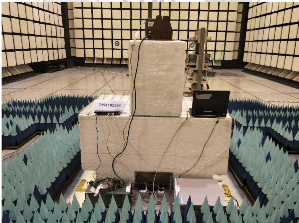
Receiver Spurious Emissions Test Setup (Rear View)
