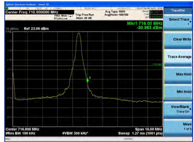
LTE Band 12 QPSK 10MHz CH-High, 1 RB
