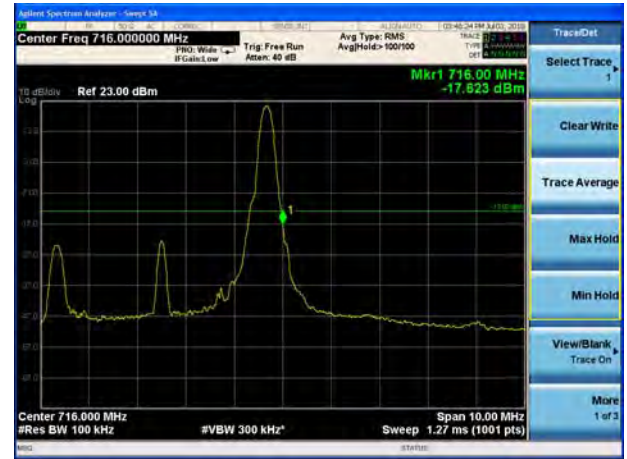
LTE Band 12 QPSK 5MHz CH-High, 100%RB
