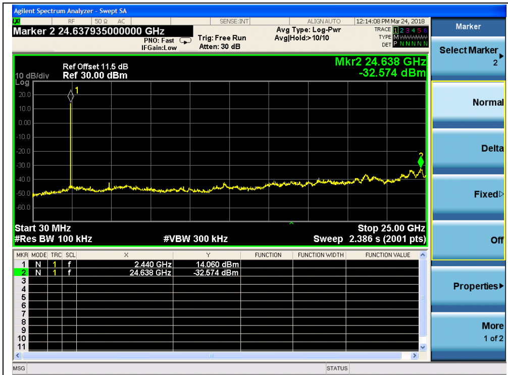
(Plot B.1: Channel = 19, 30MHz to 25GHz)
