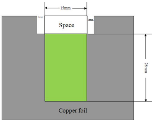
Figure 7-2 Installation 1
