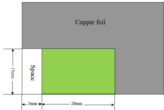
Figure 7-3 Installation 2
