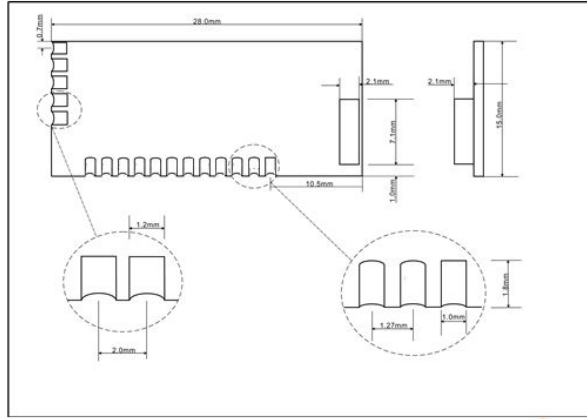
Figure 7-1 Mechanical drawing and installation
