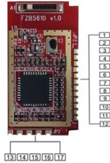
Figure 3-1 FZB5610 Module
