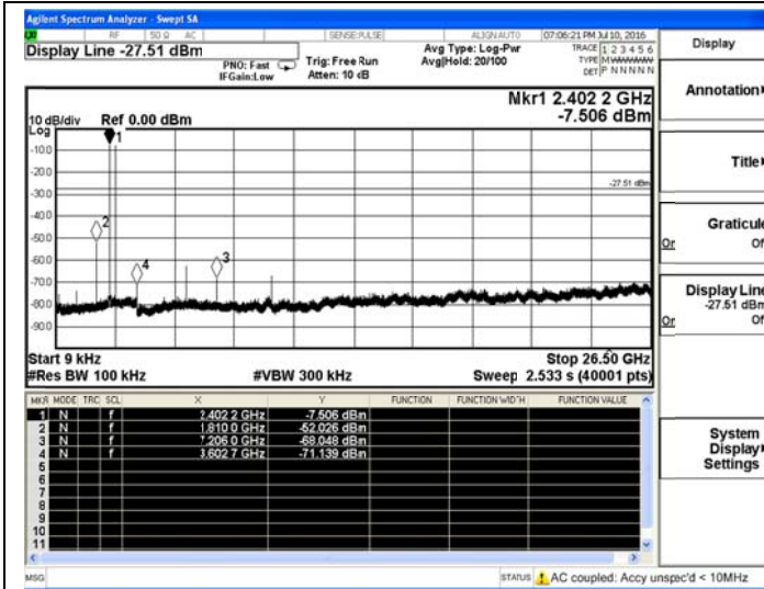
BT V4.0-Low Channel, 2402MHz
