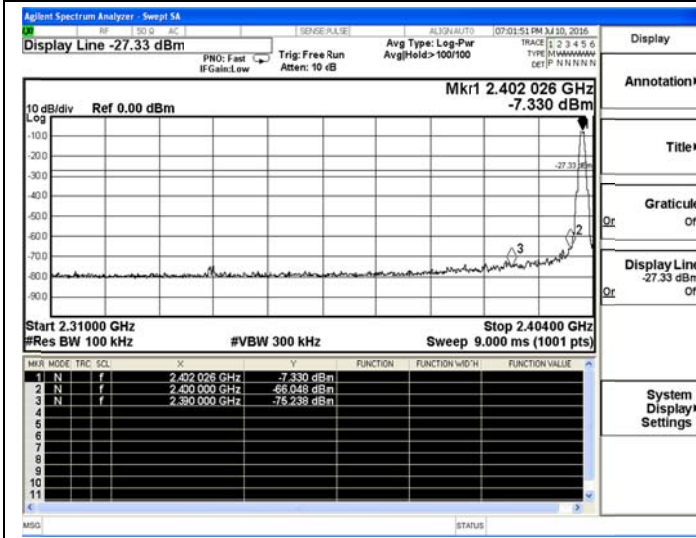
BT LE-Low Channel, 2402MHz
