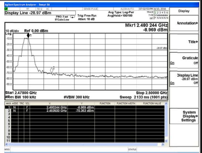
BT LE-High Channel, 2480MHz
