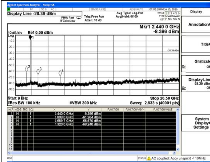
BT V4.0-Middle Channel, 2440MHz
