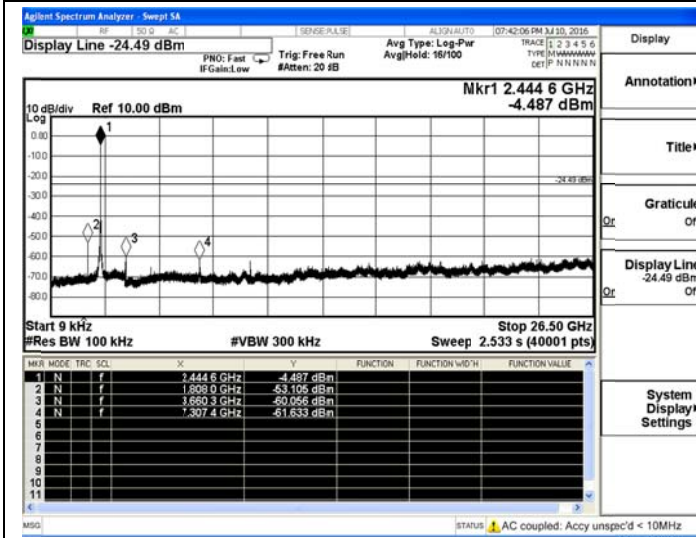
802.11n-HT20-Middle Channel, 2437MHz
