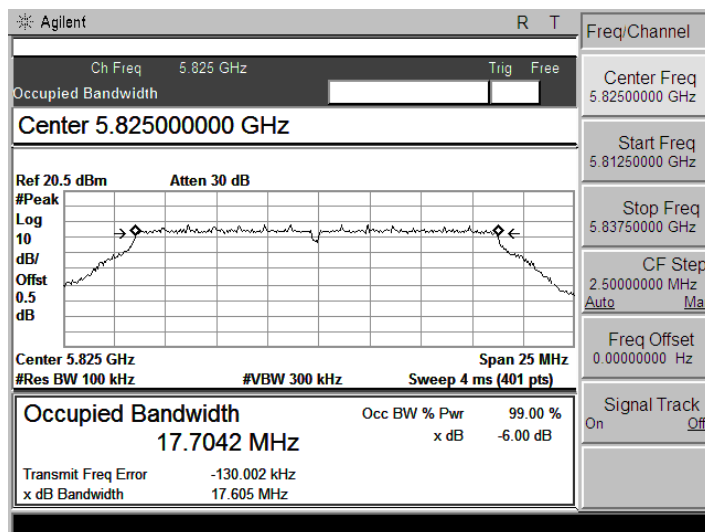
5825 MHz
