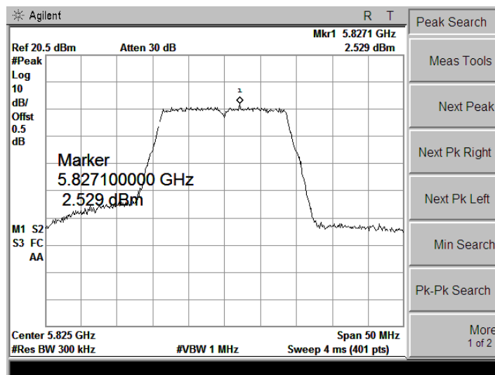
5825 MHz
