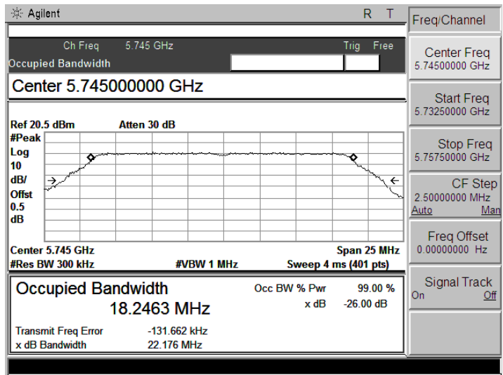
5745 MHz
