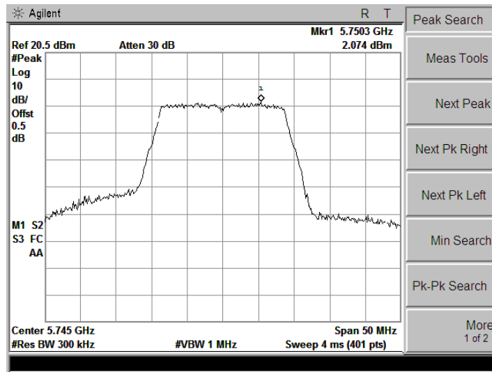
5745 MHz
