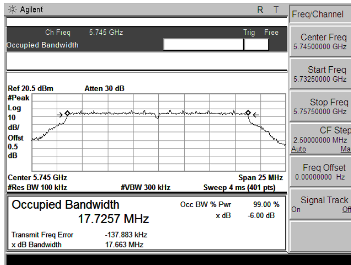
5745 MHz
