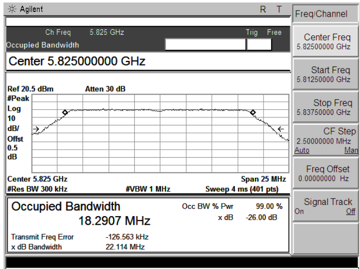
5825 MHz
