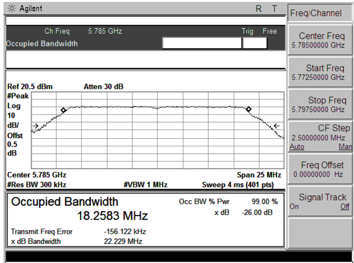
5785 MHz
