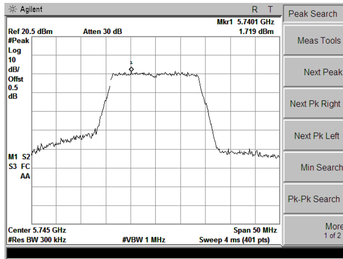
5745 MHz
