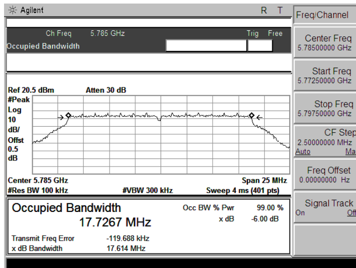
5785 MHz
