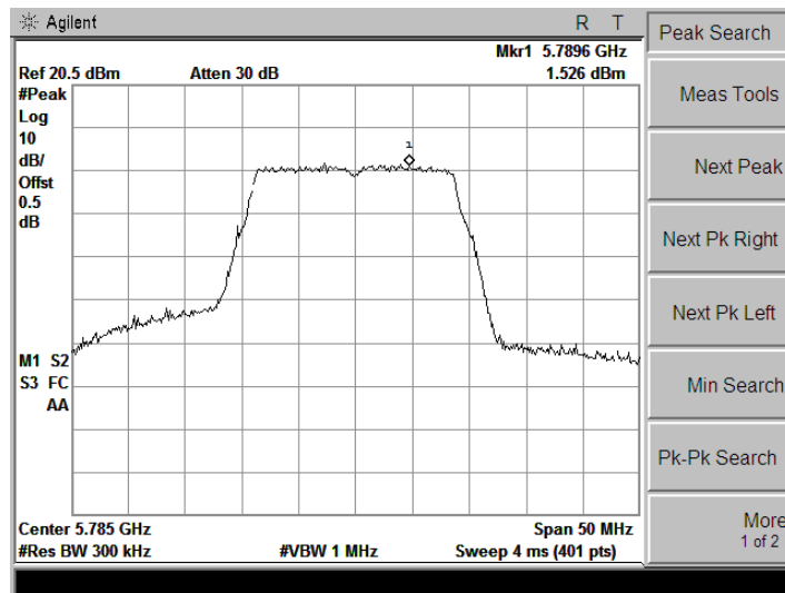
5785 MHz
