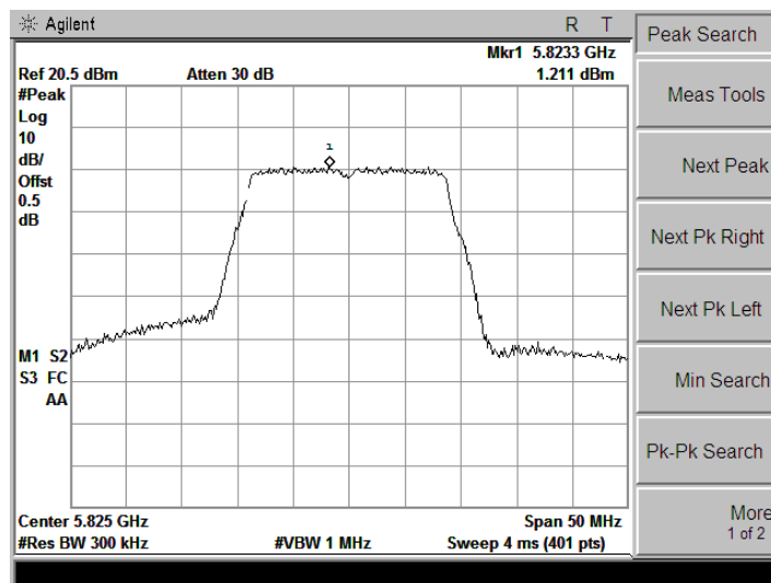
5825 MHz
