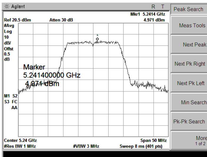
5240 MHz
