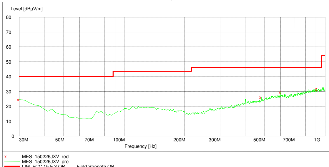
30MHz~1GHz, Horizontal
