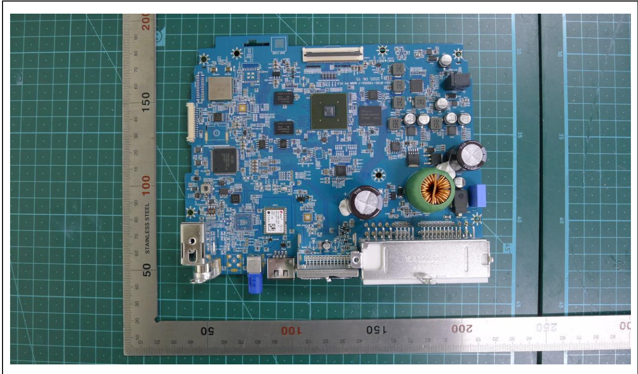
Main Board Front
