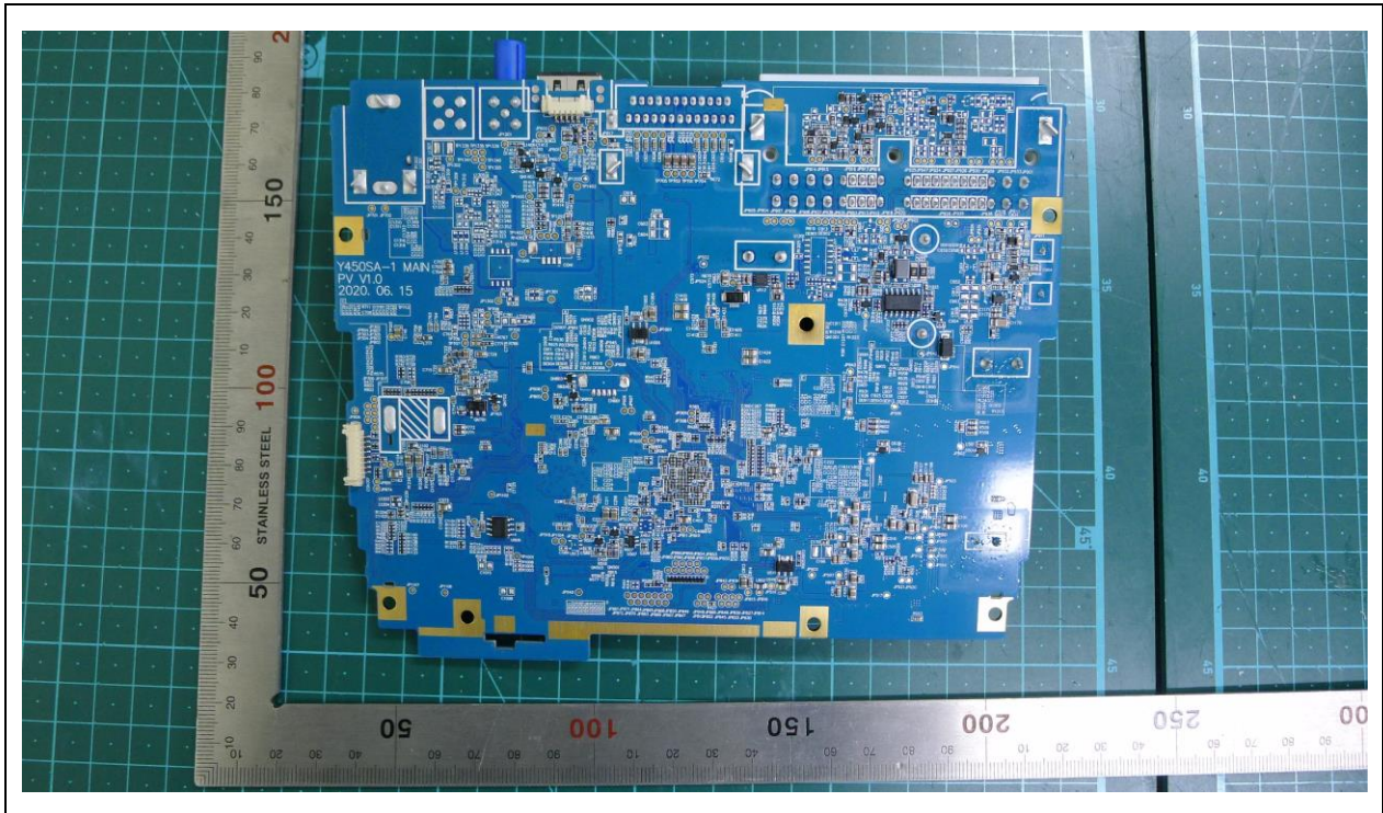
Main Board Rear
