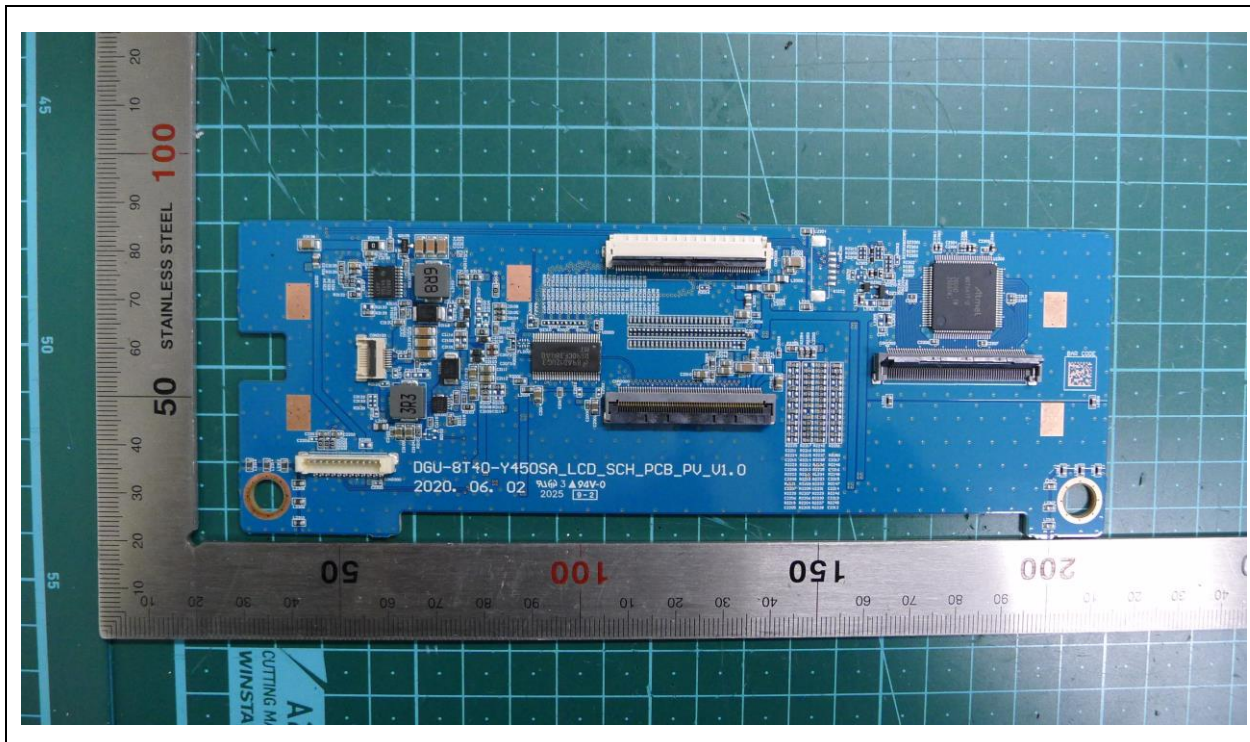
LCD Board Front
