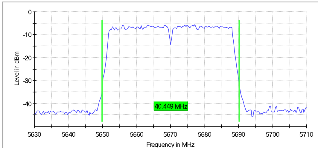
26 dB Bandwidth
