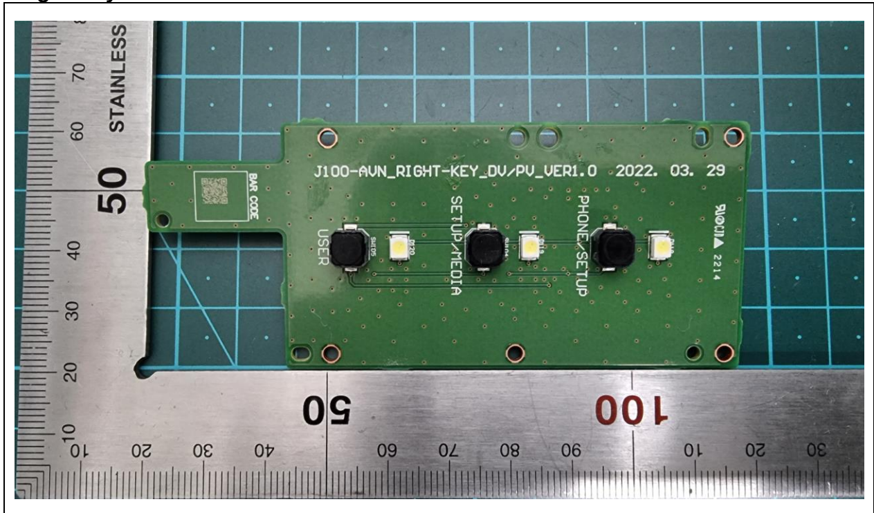
Right Key PCB Front
