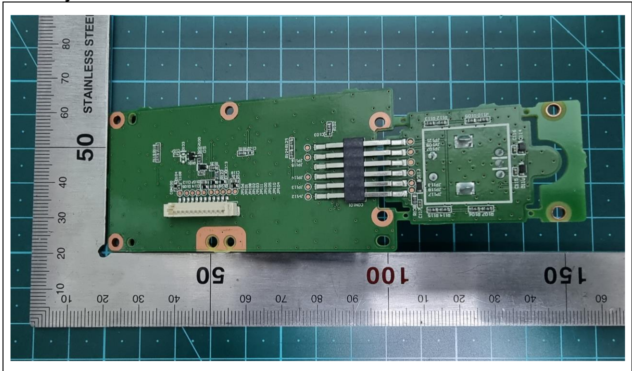
Left Key PCB Rear
