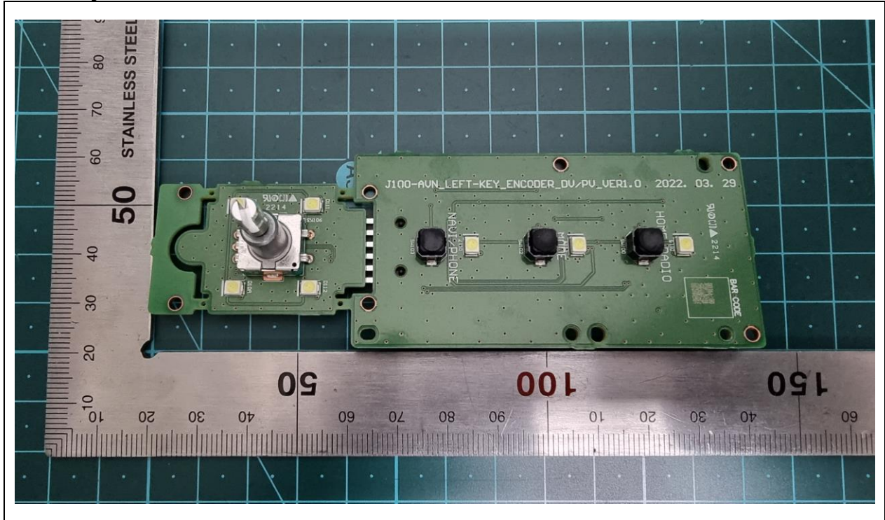
Left Key PCB Front
