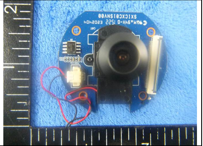
Camera Board - Front View
