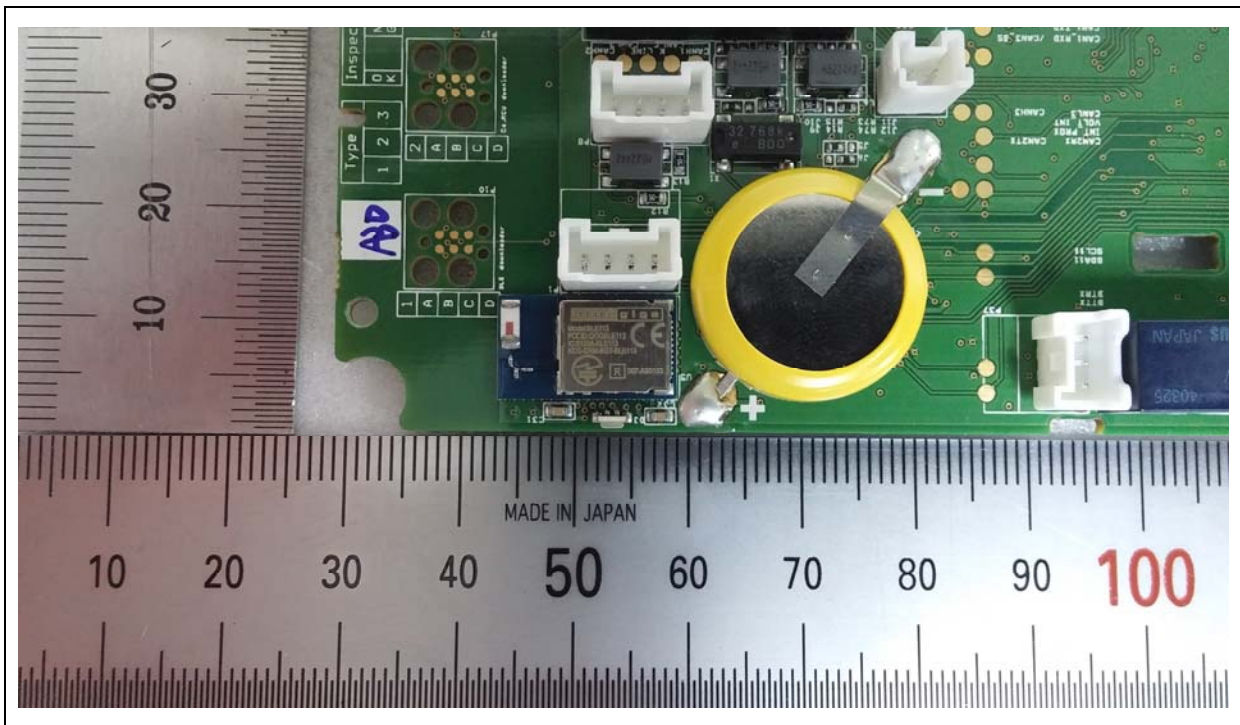
<BT Antenna>
