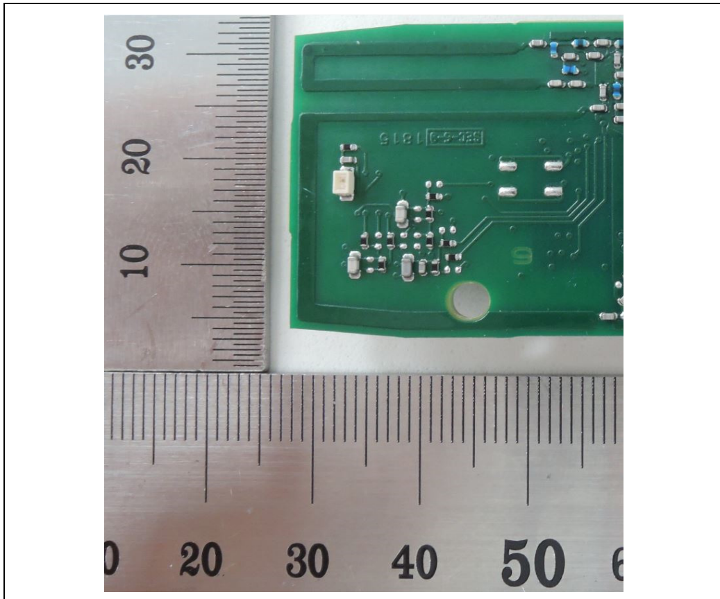
<RCK Antenna>
