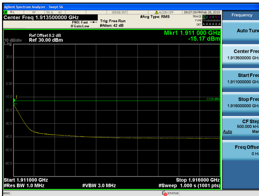
LTE Band 2 / 1.4MHz / 16QAM- RB Size/Offset (1/2)
