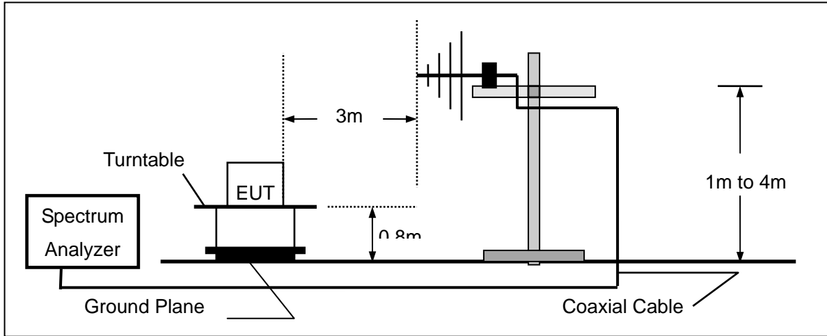
TEST SETUP OF SUBSTITUTION METHOD
