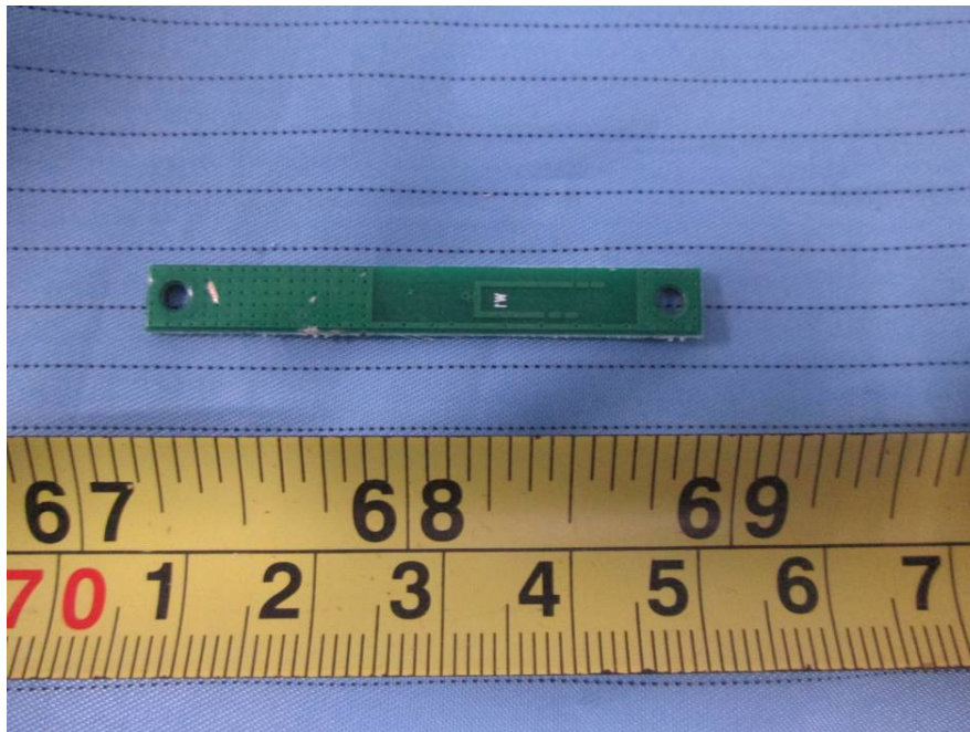
EUT – BT & GPS Antenna Bottom View
