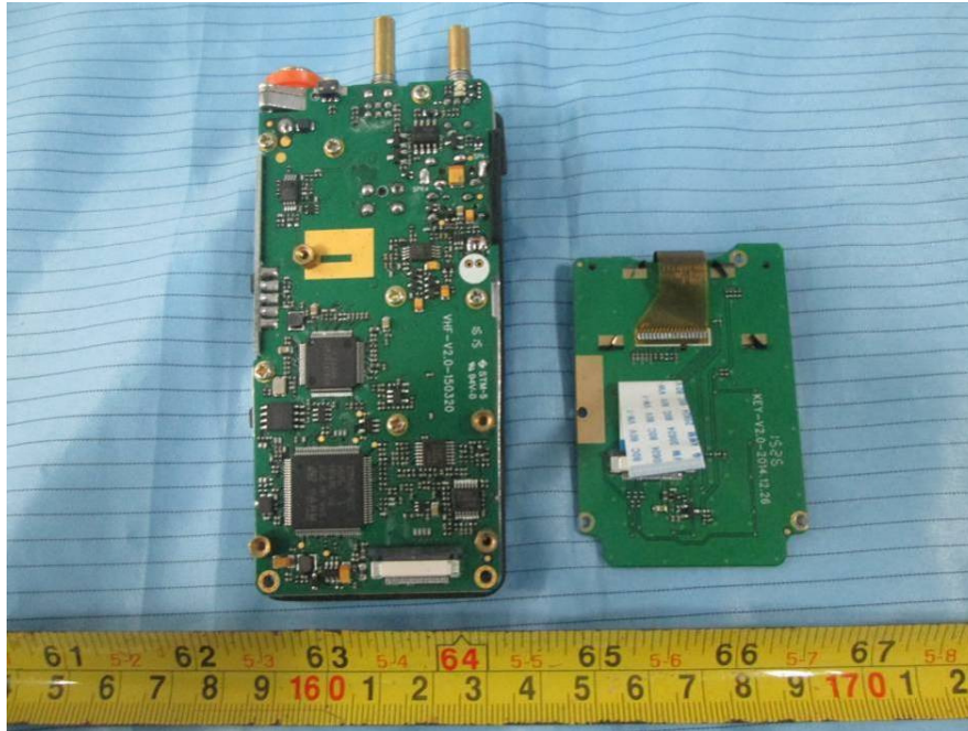
EUT – Cover off 3 View
