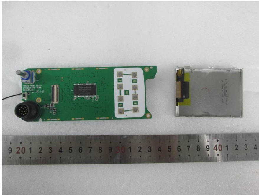
EUT – Main Board Bottom 2 Shilding off View
