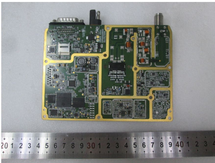
EUT – Main Board Bottom 1 Shilding off View
