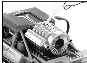
Open the water injection port and fill with clean water.
