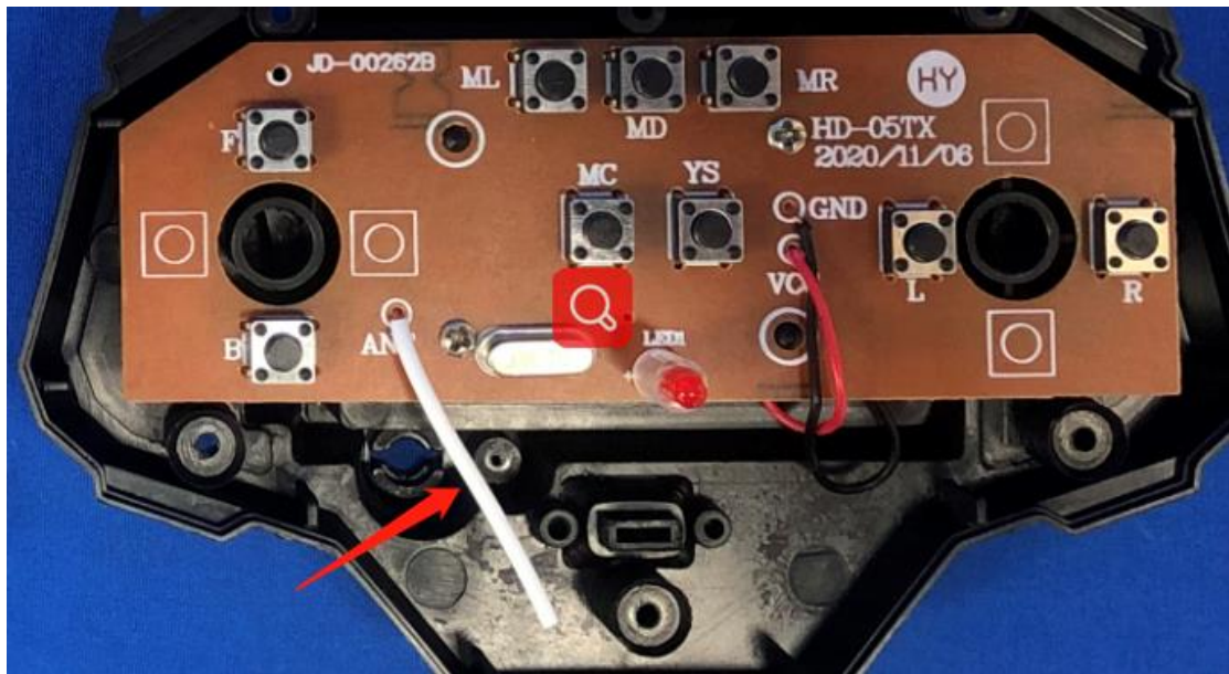
Antenna length: 3.1cm
