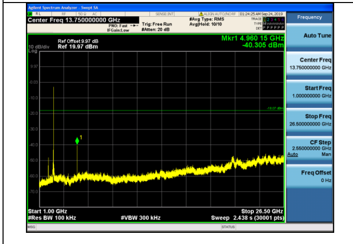
\pi/4 -DQPSK on Channel 79
