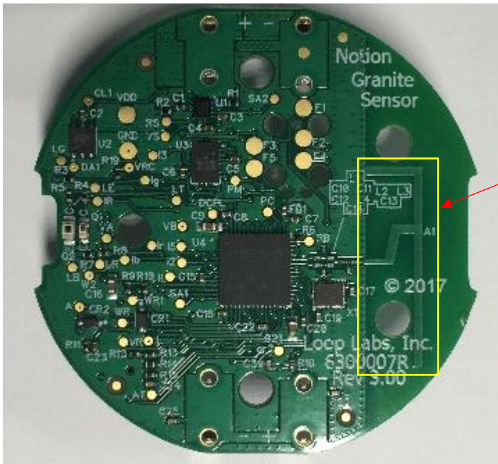
Figure 3- Granite Sensor Model 007, Top Side
