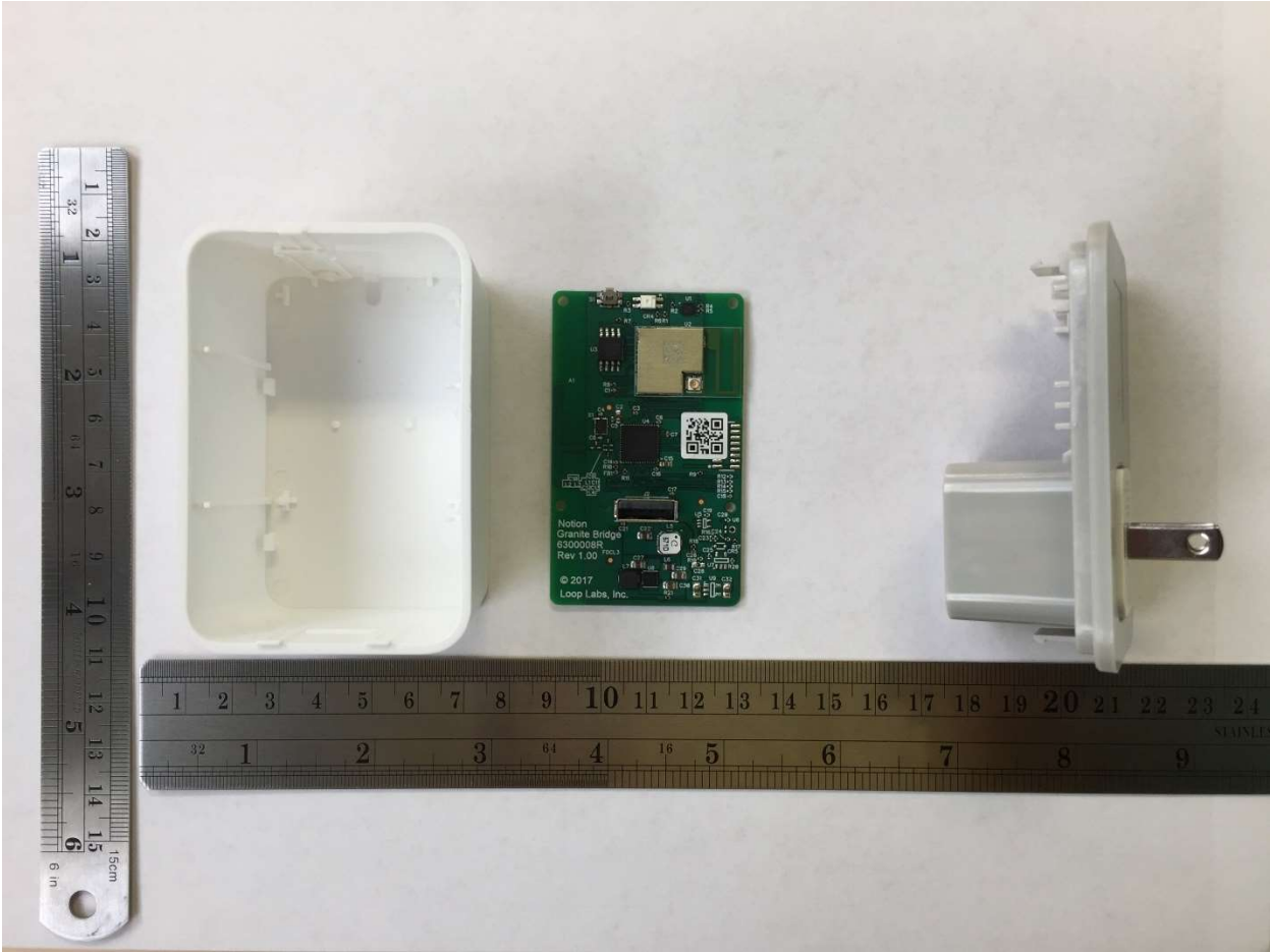
Figure 1- Disassembled View
