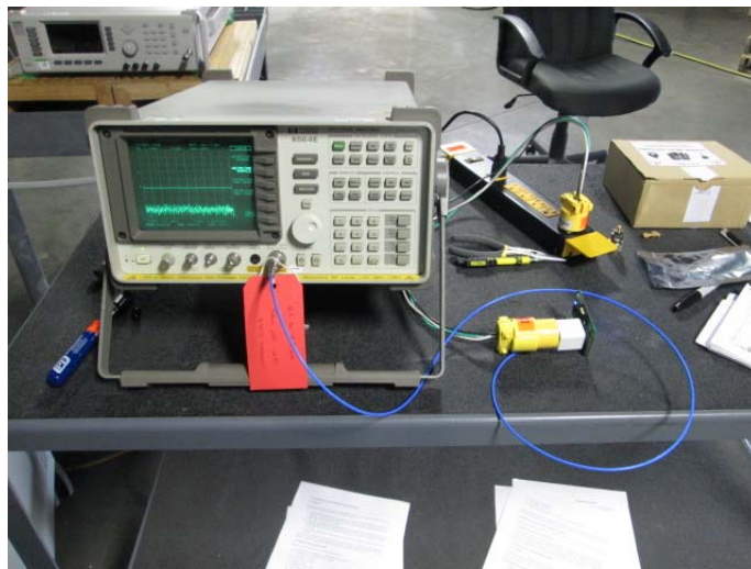
Test Setup – Conducted Measurements – Antenna Port
