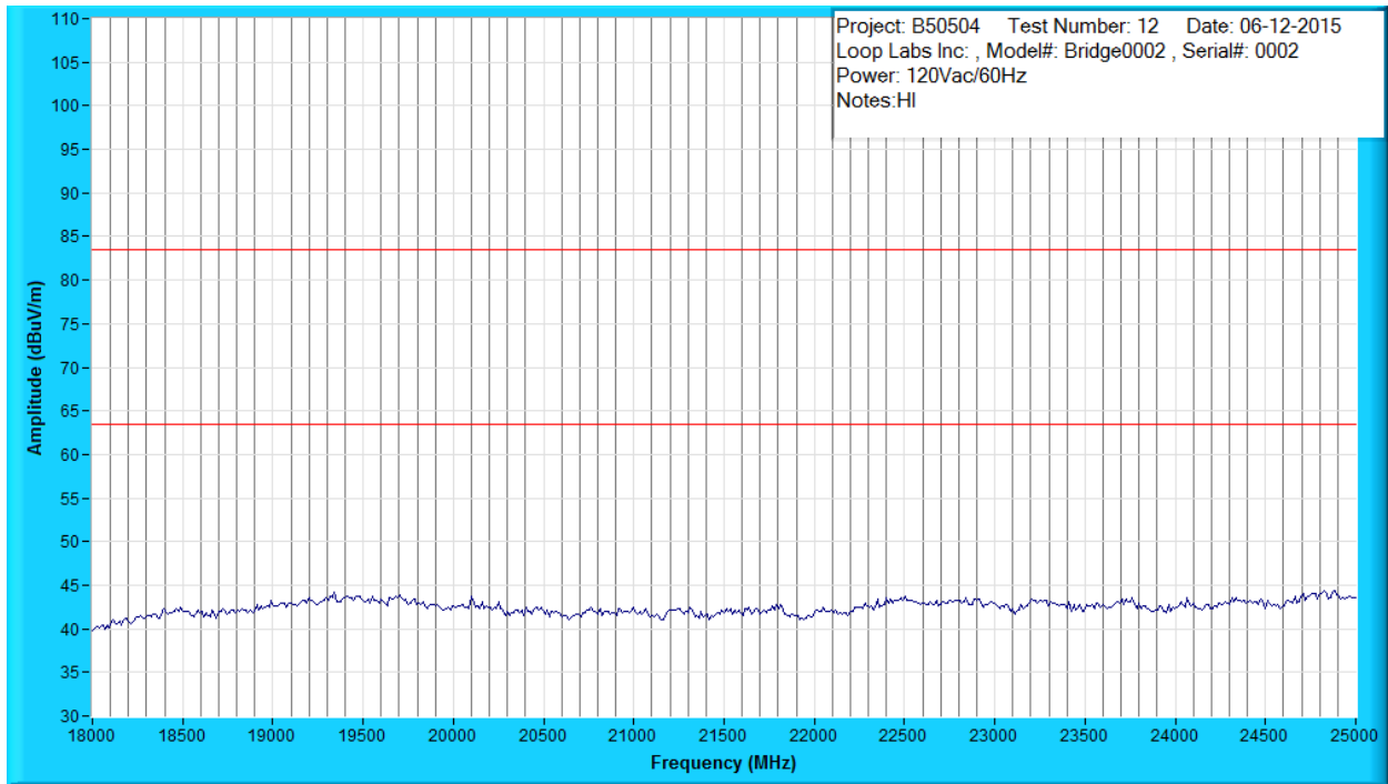
Figure A14: Radiated Emissions Prescan, 18GHz to 25GHz, Peak Measurements at 1m Distance, MID
