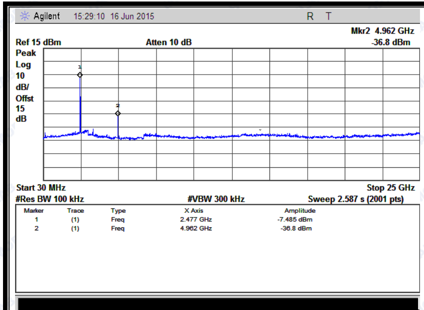
(Plot I.1: Channel = 78, 30MHz to 25GHz @ 8-DPSK)
