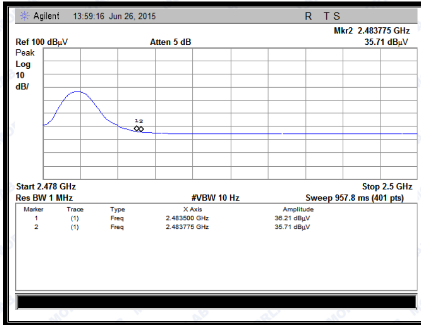
(Plot F2:Channel = 78 AVERAGE @ 8-DPSK Mode)
