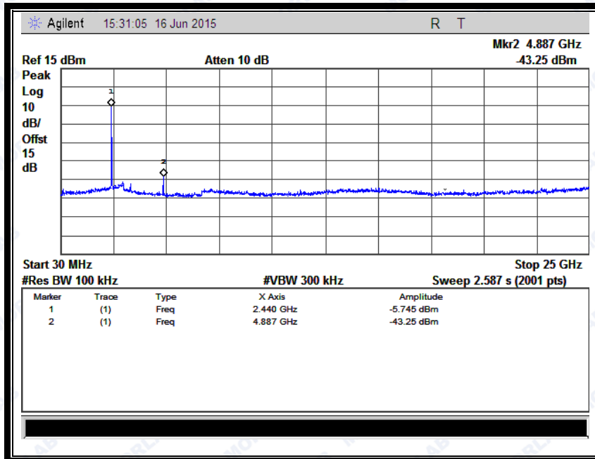
(Plot H.1: Channel = 39, 30MHz to 25GHz @ 8-DPSK)
