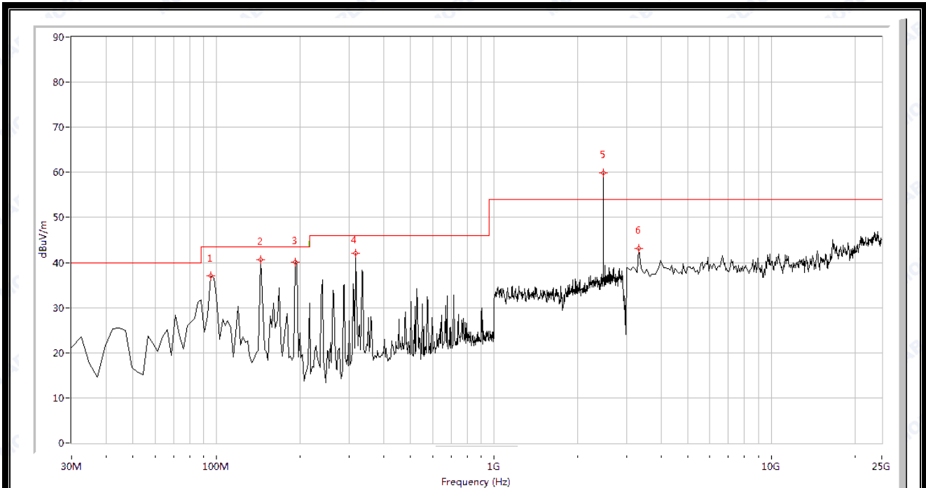
Plot for Channel = 78
