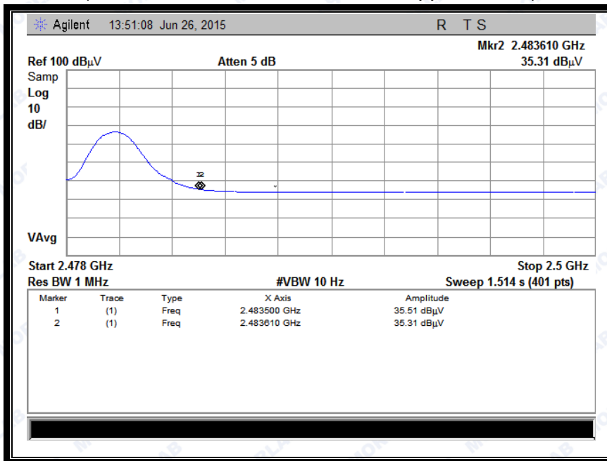
(Plot D2: Channel = 78 AVERAGE @ \pi/4 -DQPSK)
