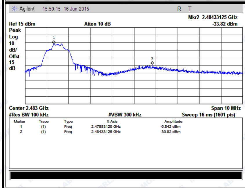
(Plot I.1: Channel = 78, Band edge @ 8-DPSK)
