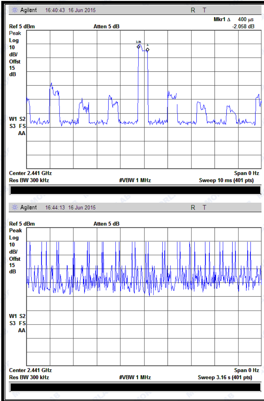
(Plot D: DH1 @ π/4-DQPSK)
