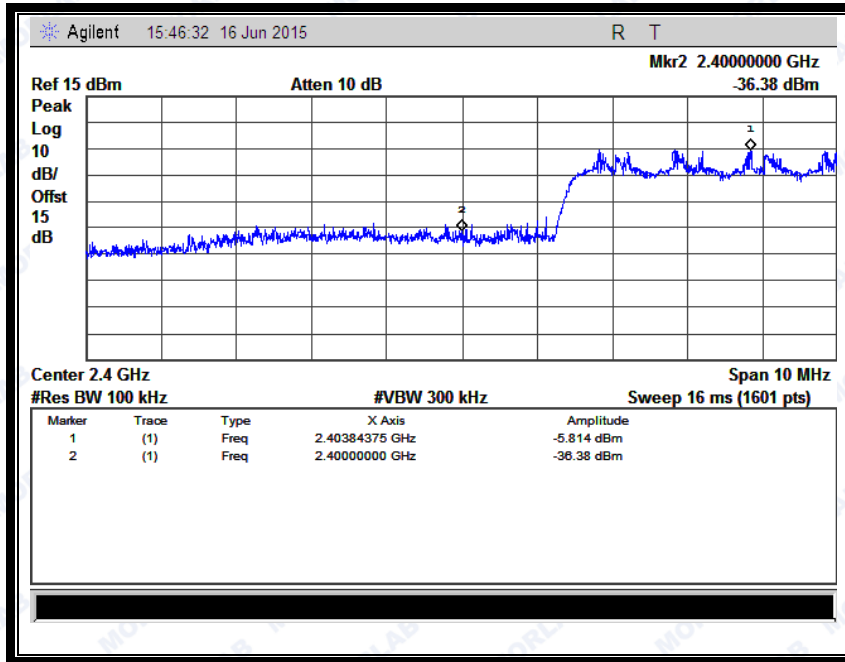
(Channel = 0, Band edge with hopping on @ 8-DPSK)
