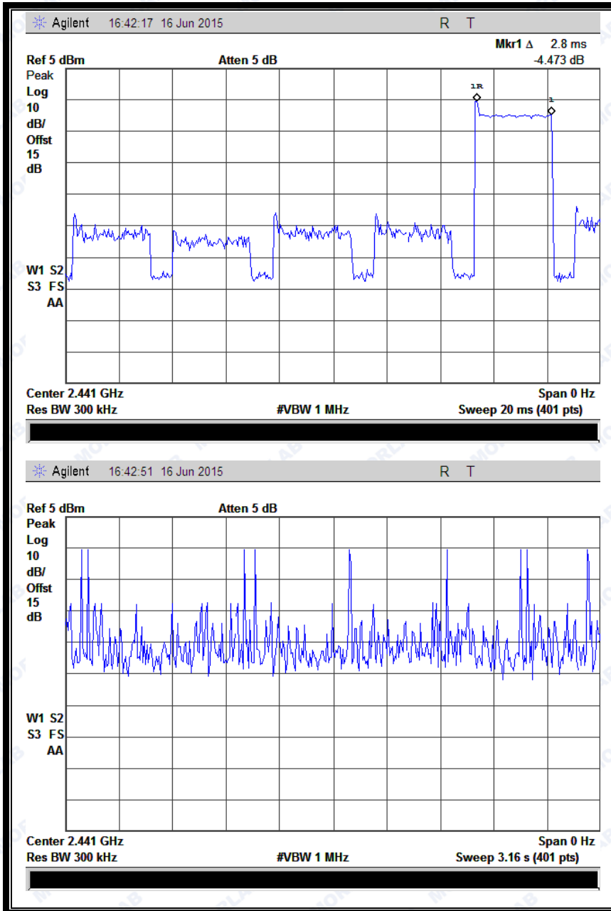
(Plot F: DH5 @ π/4-DQPSK)
